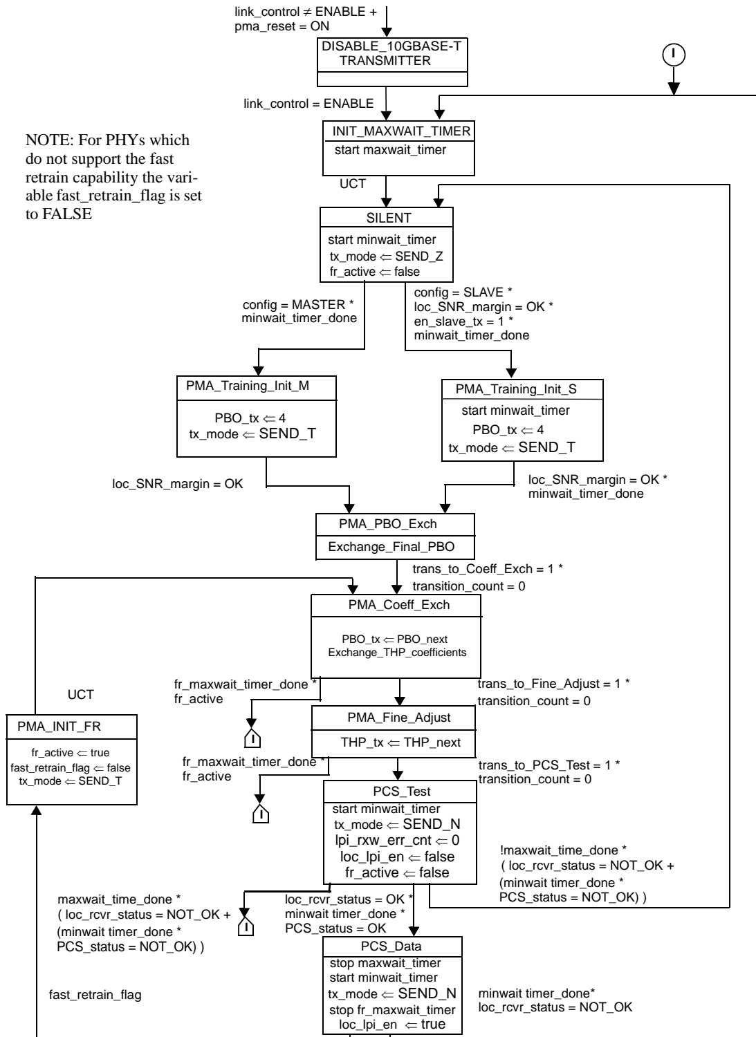
Figure 55-24—PHY Control state diagram
