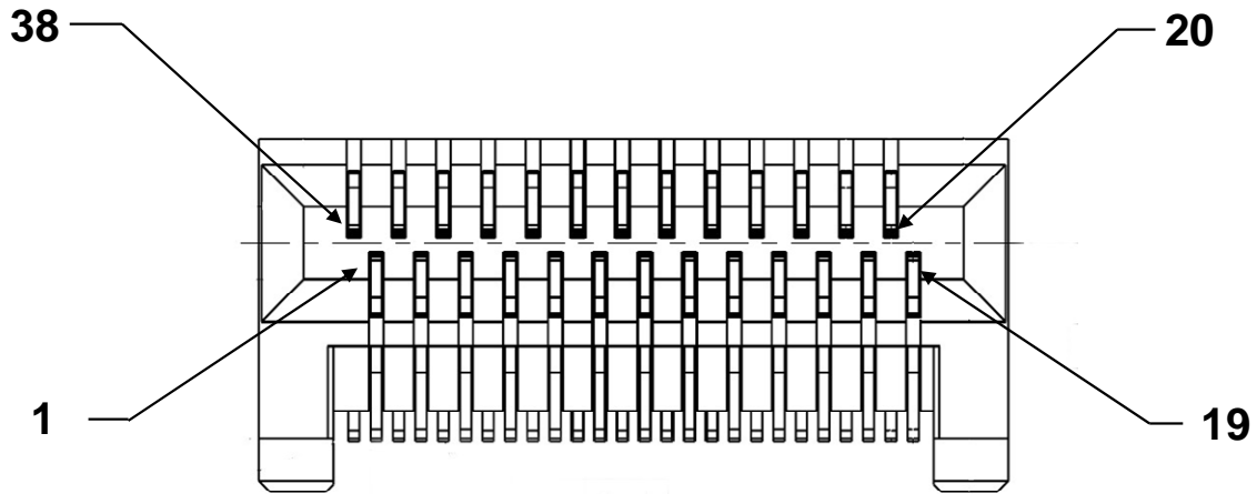
Connector Interface
