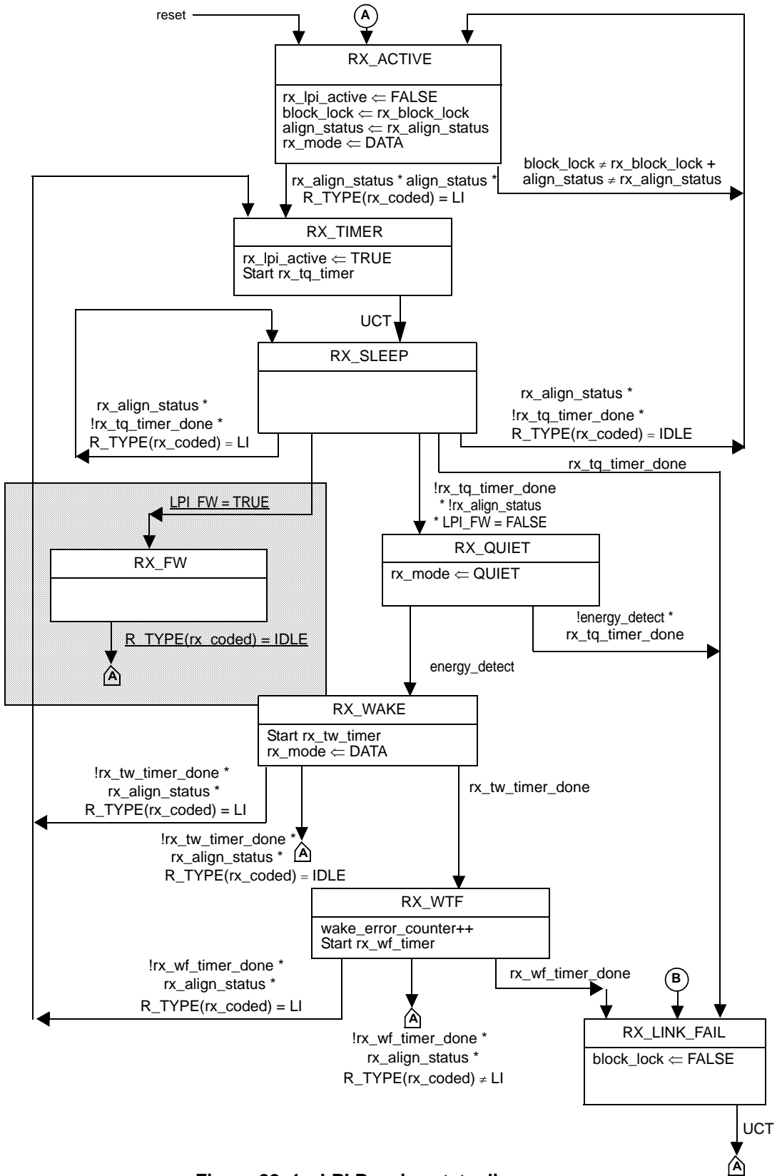
Figure 82-1—LPI Receive state diagram
