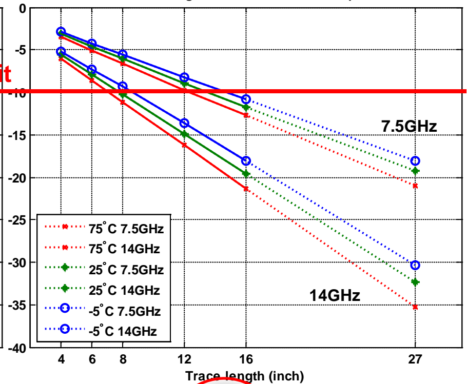
PCB A 1 5degree Rotation SDD21 Comparison
