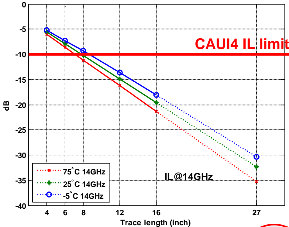
PCBA 1 5degree Rotation SDD21 Comparison
