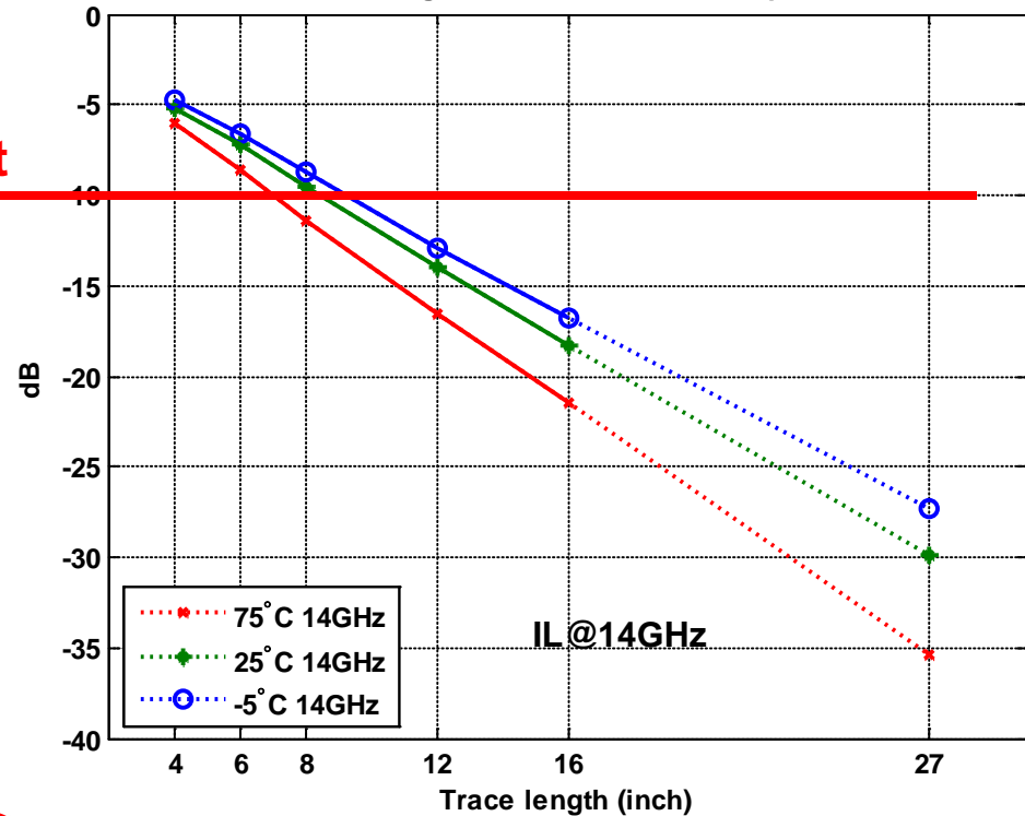
PCBA 2 5degree Rotation SDD21 Comparison
