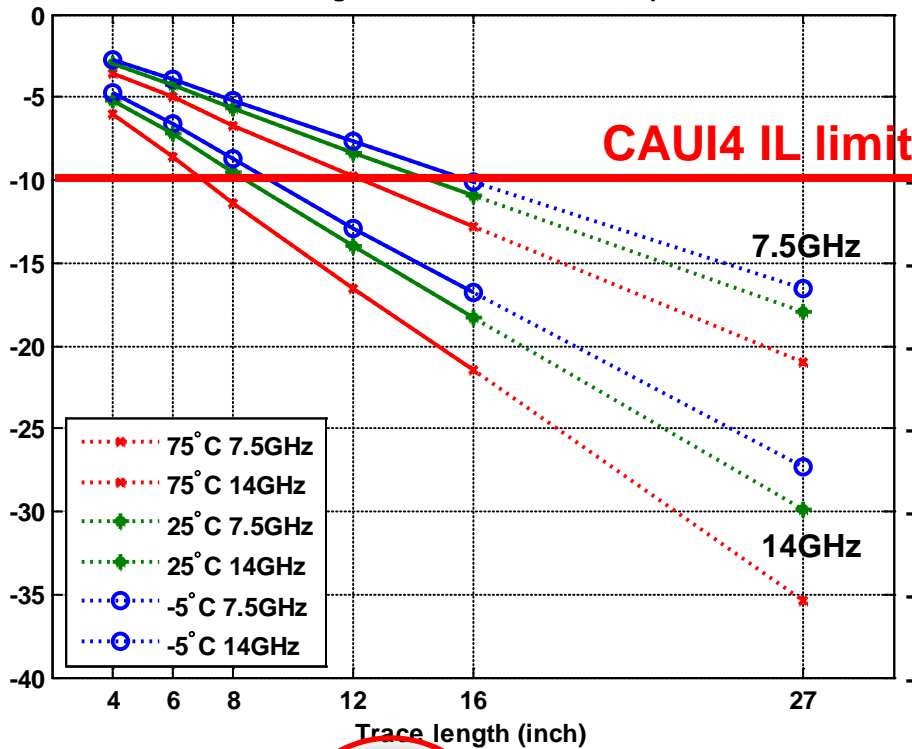
PCB A 2 5degree Rotation SDD21 Comparison
