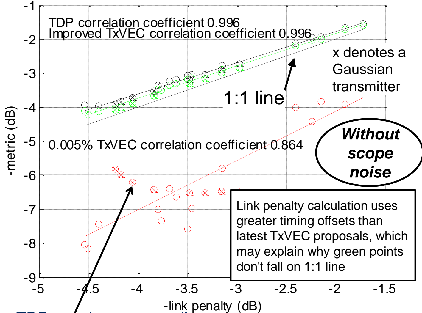
Black TDP; red TxVEC 0.005%; green soft TDP = improved TxVEC
