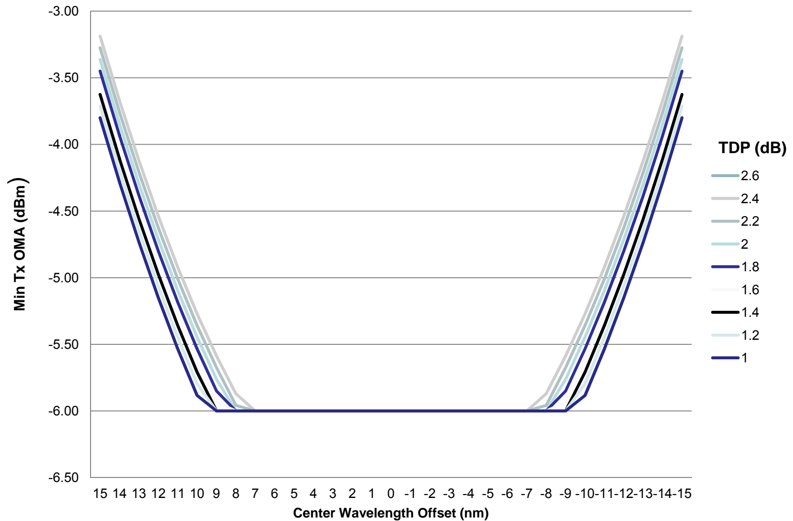
Figure 1: 100GBASE-nR4 minimum transmit OMA as a function of 1310nm center wavelength offset and TDP
