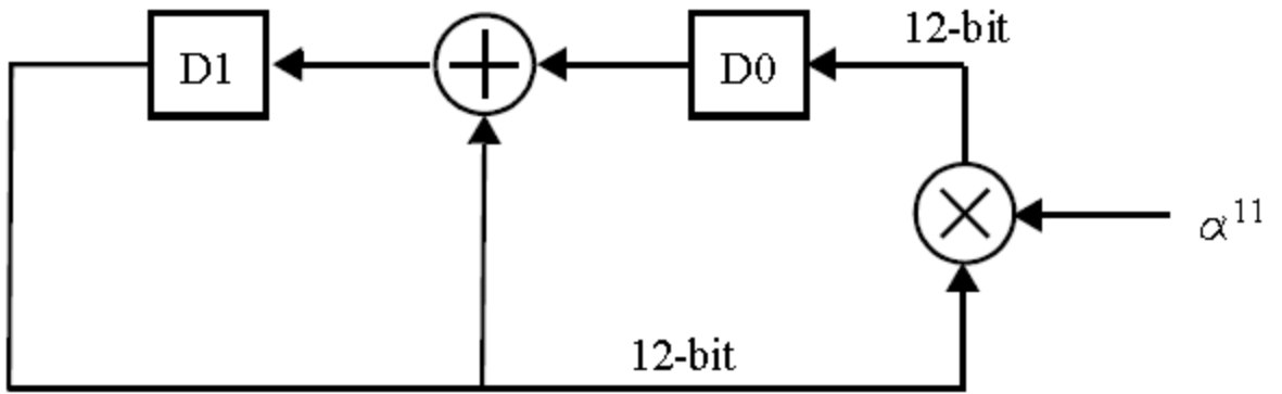
Figure 102-6—PHY-Link scrambler
