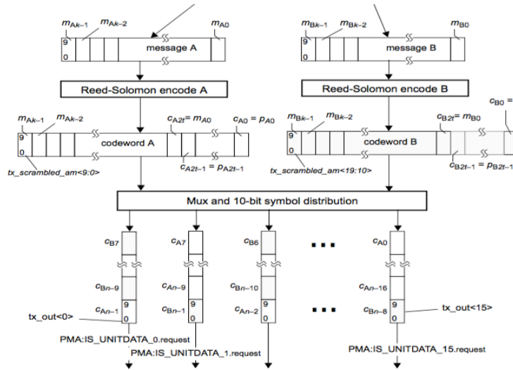
Figure 119-11—400GBASE-R Transmit bit ordering
