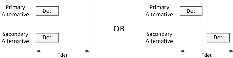
Figure 145B-X1—Parallel detection
