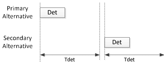
Figure 145B-X2—Staggered detection
