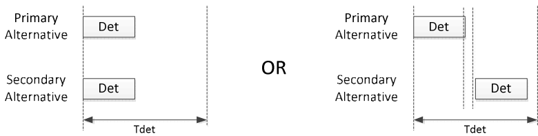
Figure 145-X—Parallel detection
