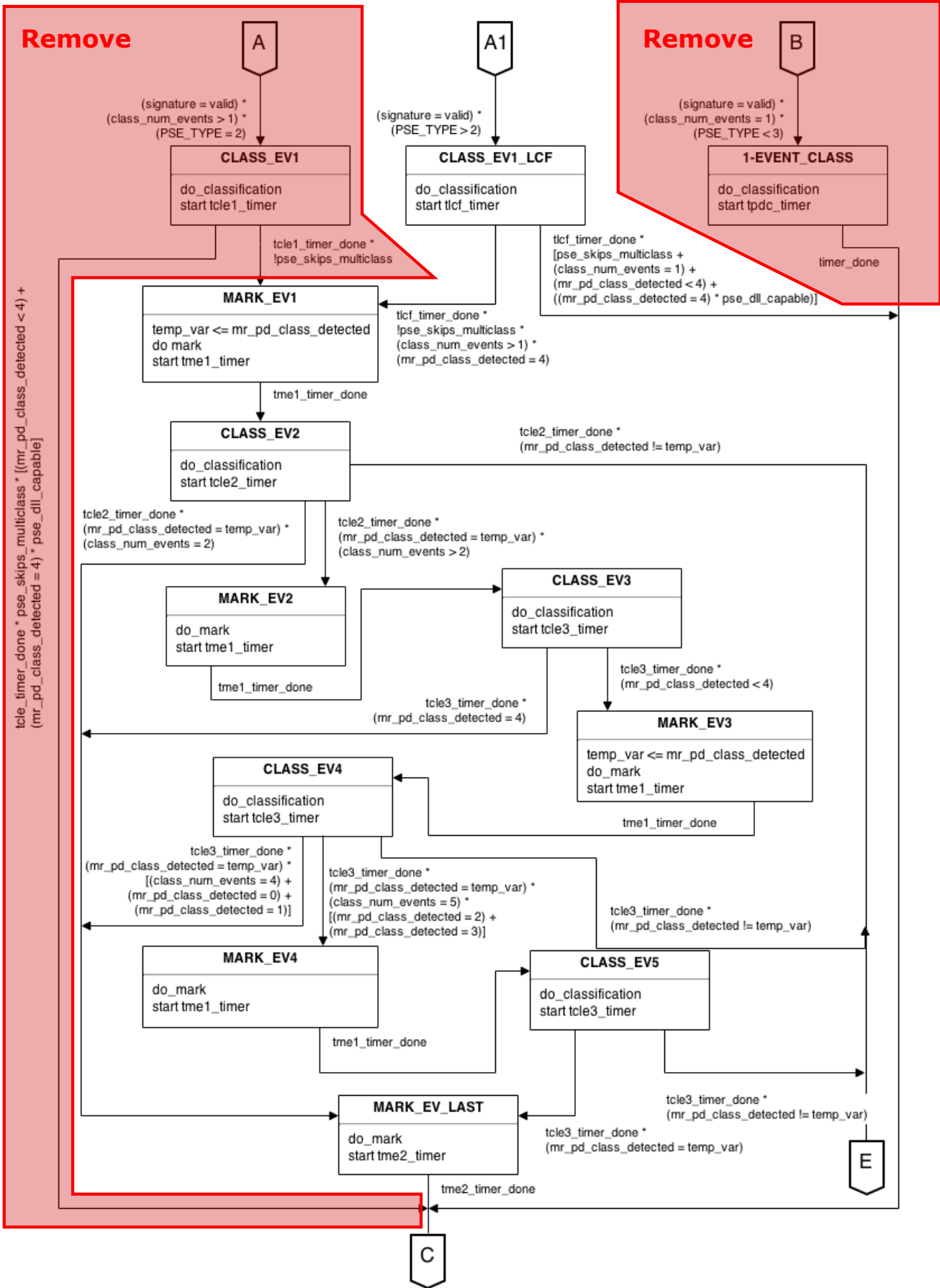
Figure 33-9g—Type 3 and Type 4 PSE classification state diagram
