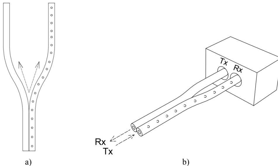
Figure 2: a) Duplex POF cable splitting, b) 1000BASE-H MDI receptacle to POF cable connection
