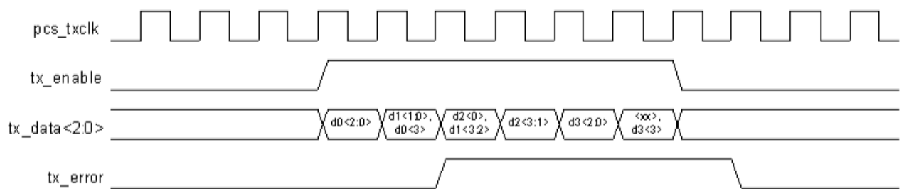
Case 2: 4B3B MII signals conversion ((3n+1)-bit data, 2 stuff bits appended)
