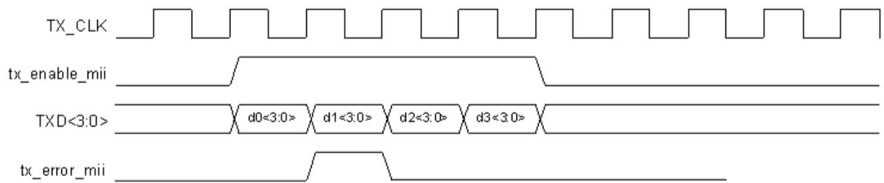
Case 1: 4B3B MII signals conversion (3n-bit data, no stuff bit appended)
