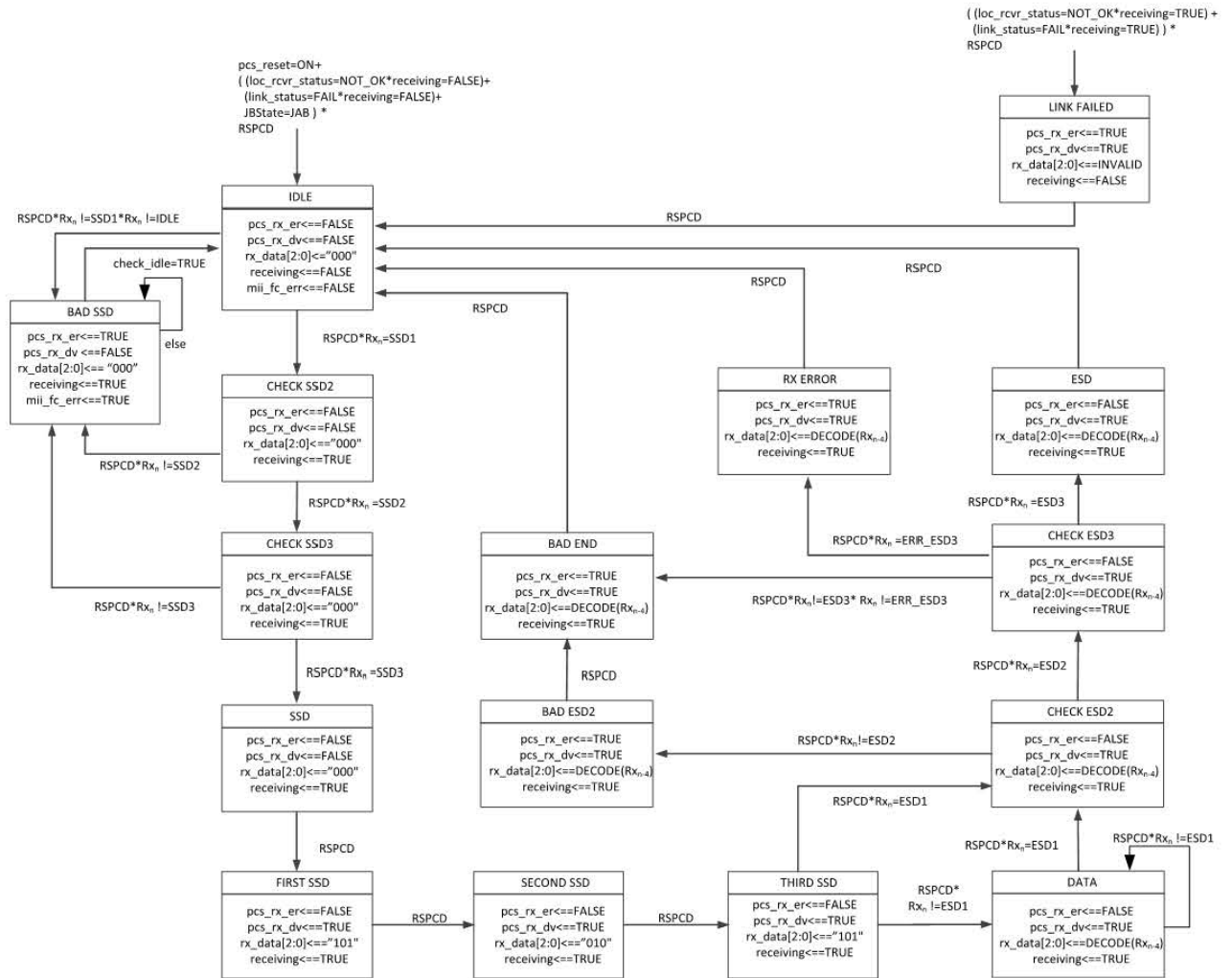
Figure 96.9---- PCS Receive State Diagram
