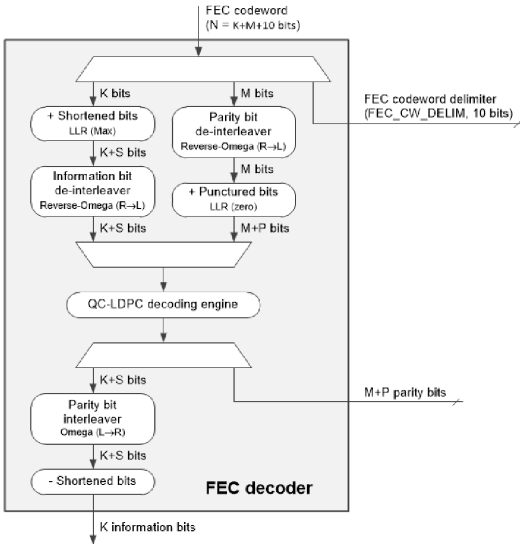
Figure 142–15 LDPC FEC Decoder
