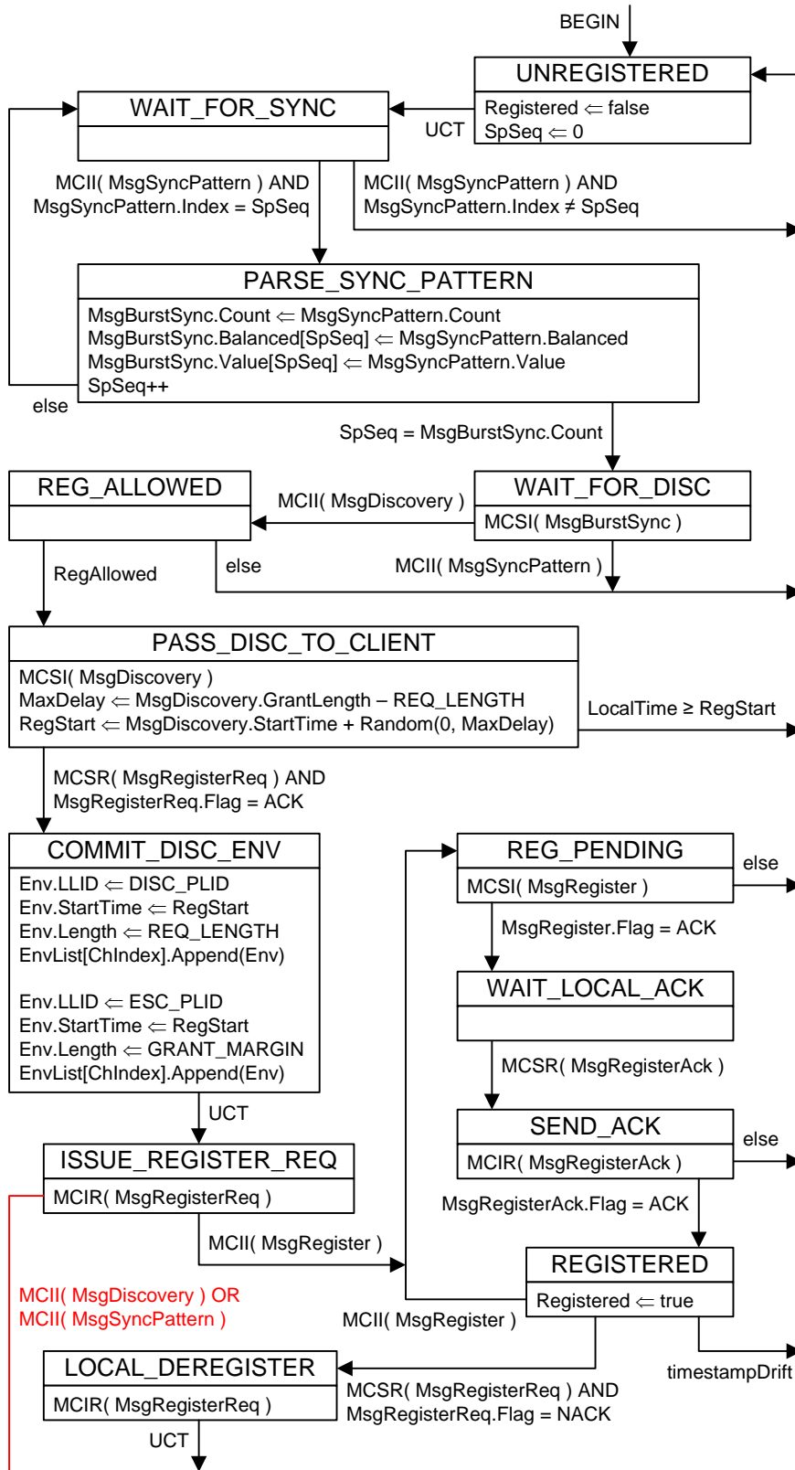
Figure 144-22 -- ONU Registration state diagram
