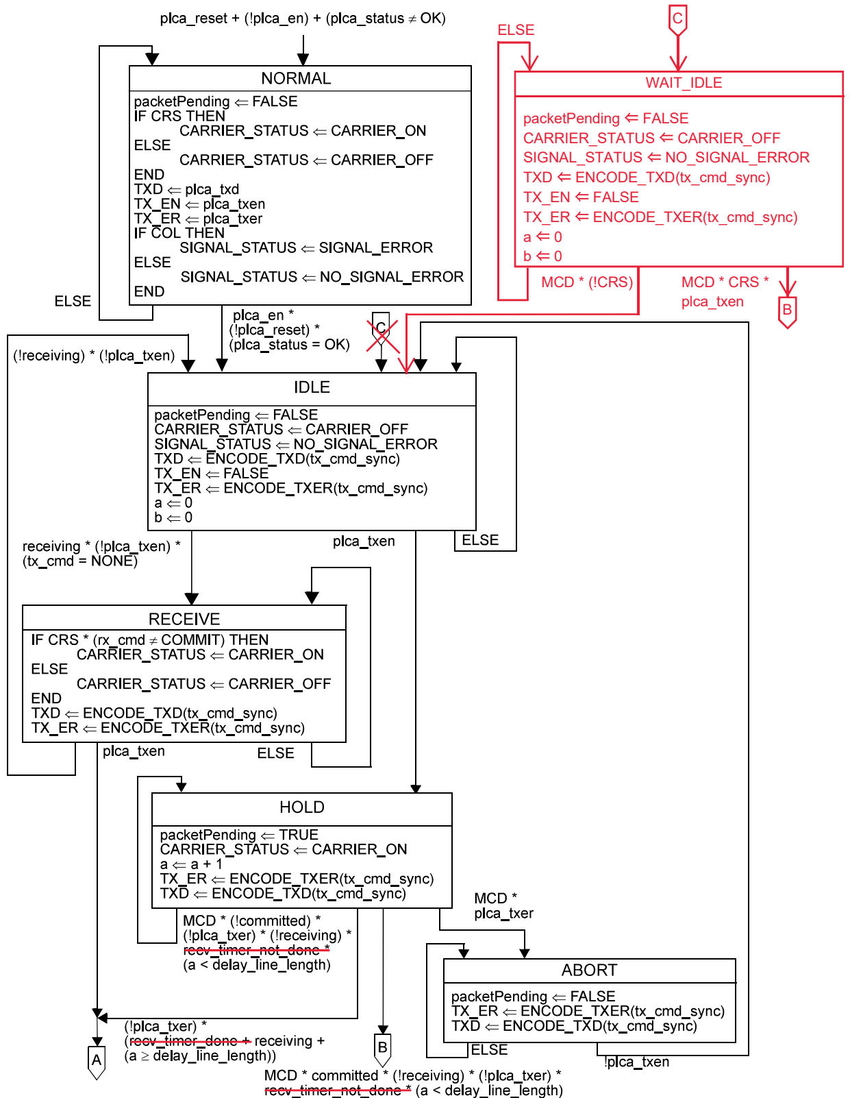
Figure 148-4—PLCA Data state diagram
