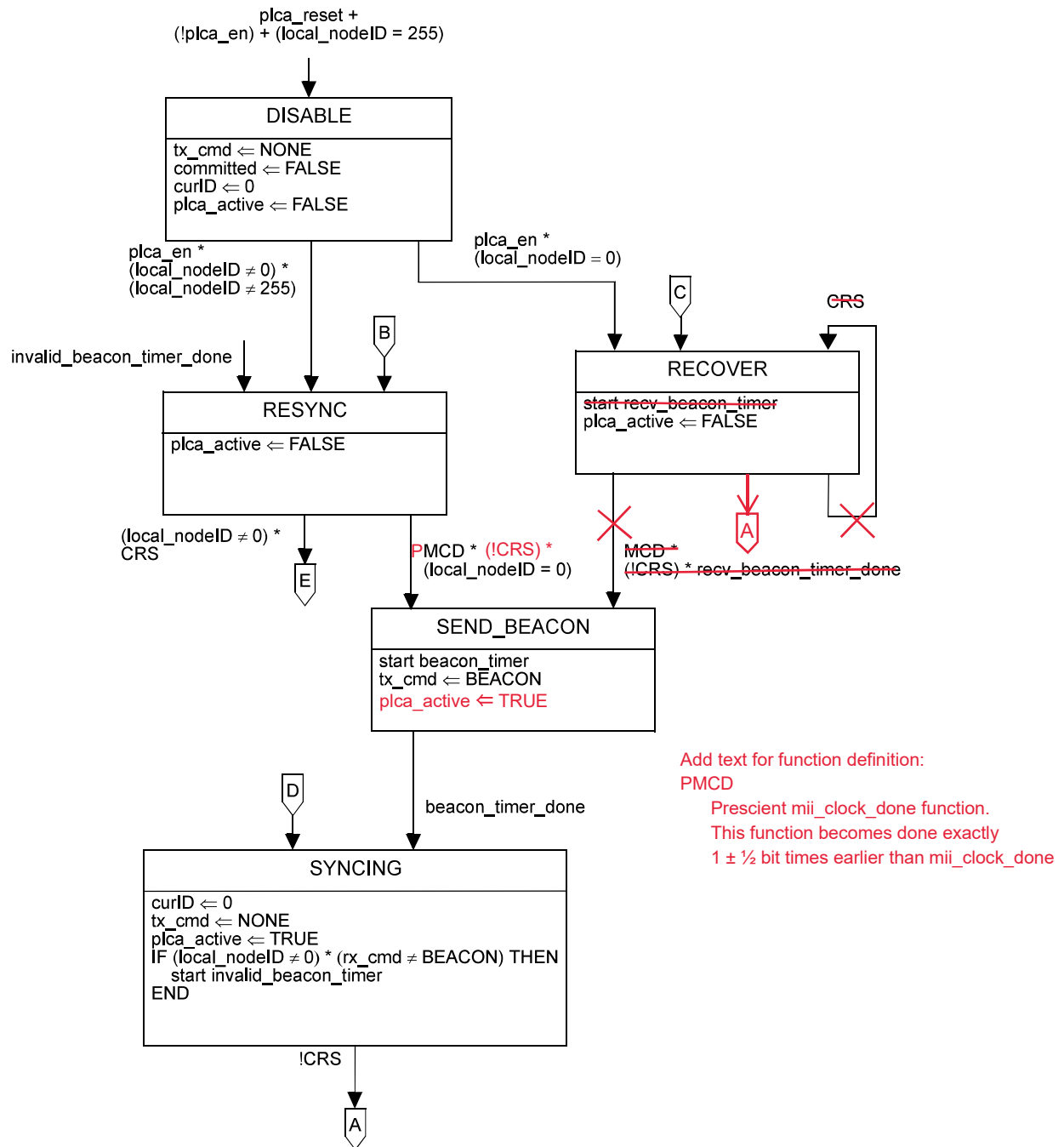
Figure 148–3—PLCA Control state diagram
