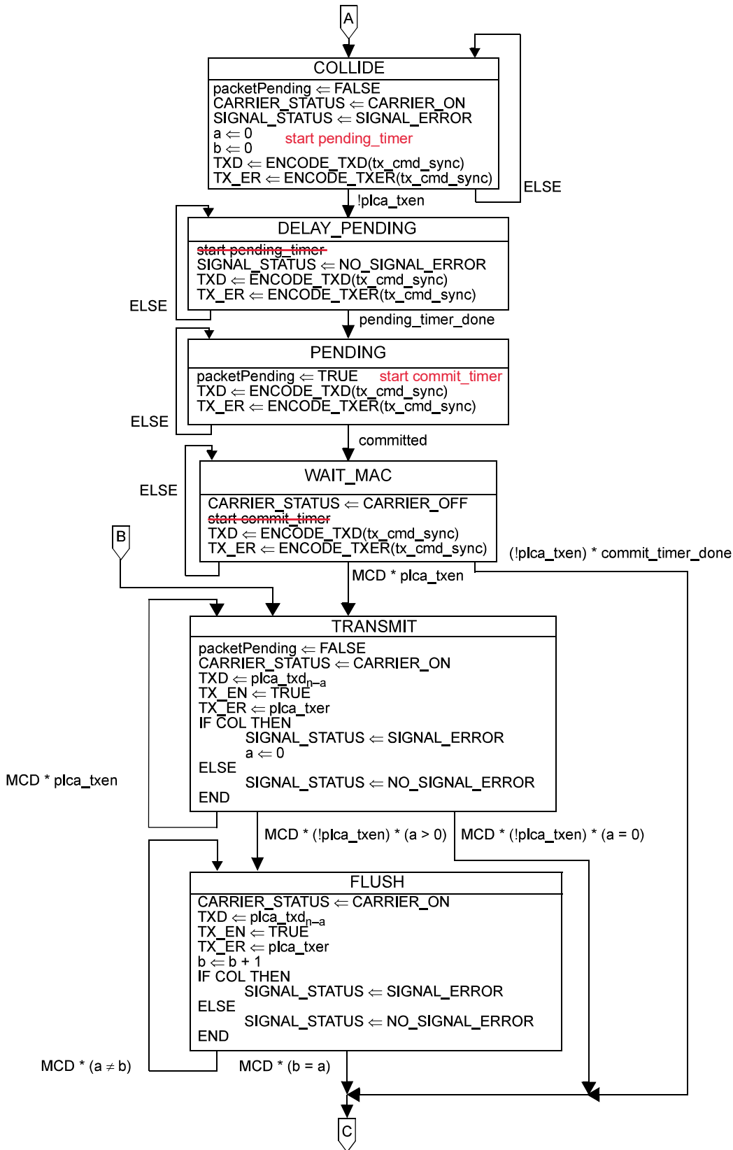
Figure 148-4—PLCA Data state diagram (continued)
