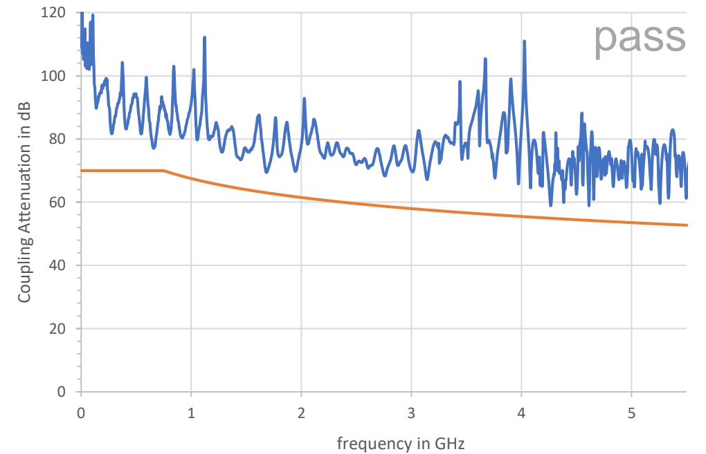
Coupling Attenuation
