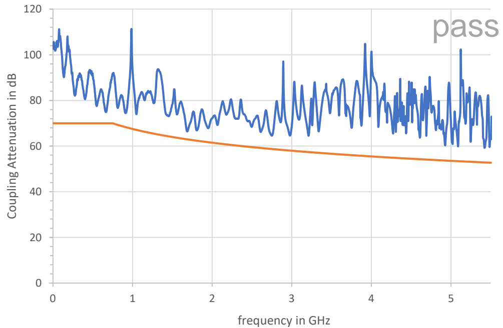
Coupling Attenuation
