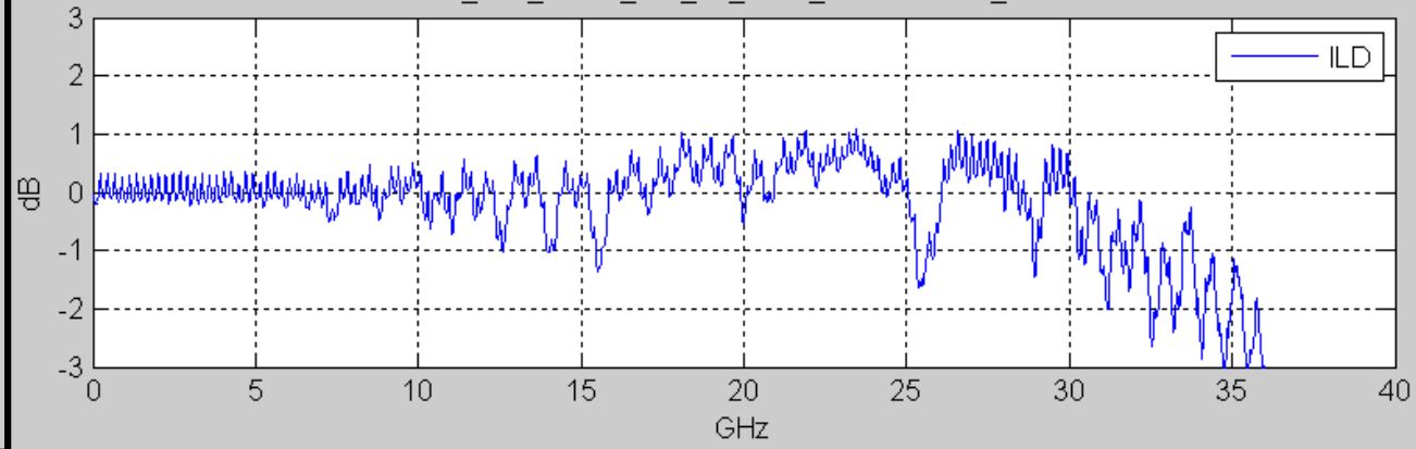
CR_eval_kareti_3ck_01_1118_ortho--OAch4_tILD
