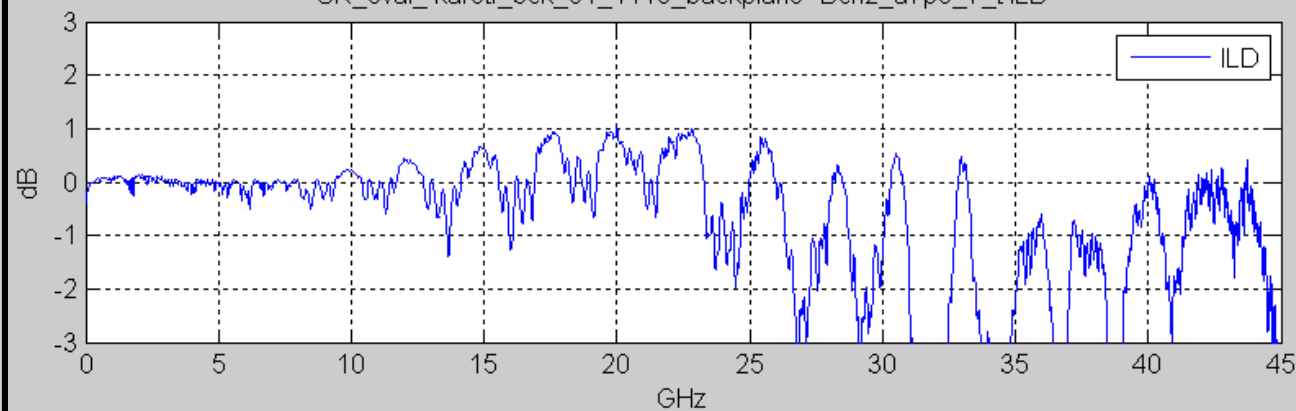
CR_eval_kareti_3ck_01_1118_backplane--Bch2_a7p5_7_tILD
