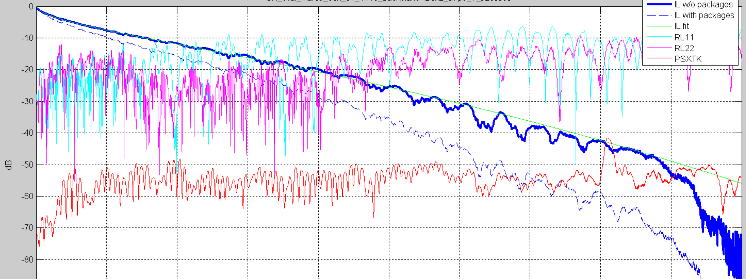
CR_eval_kareti_3ck_01_1118_backplane--Bch2_a7p5_7_tICR
