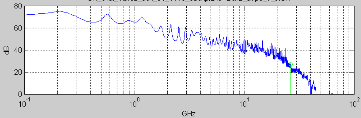
CR_eval_kareti_3ck_01_1118_backplane--Bch2_a7p5_7_tICR
