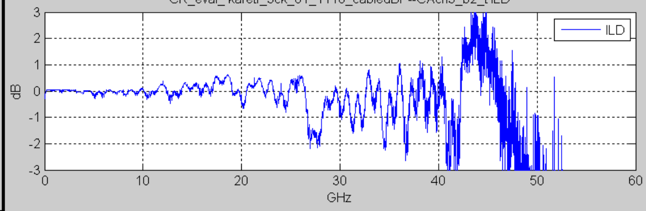
CR_eval_kareti_3ck_01_1118_cabledBP--CAch3_b2_tILD
