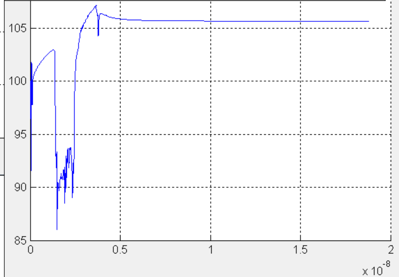
eval_tracy_DPO_12dB_backplaneChannels--DPO_4in_Meg7_THRU Rx port
