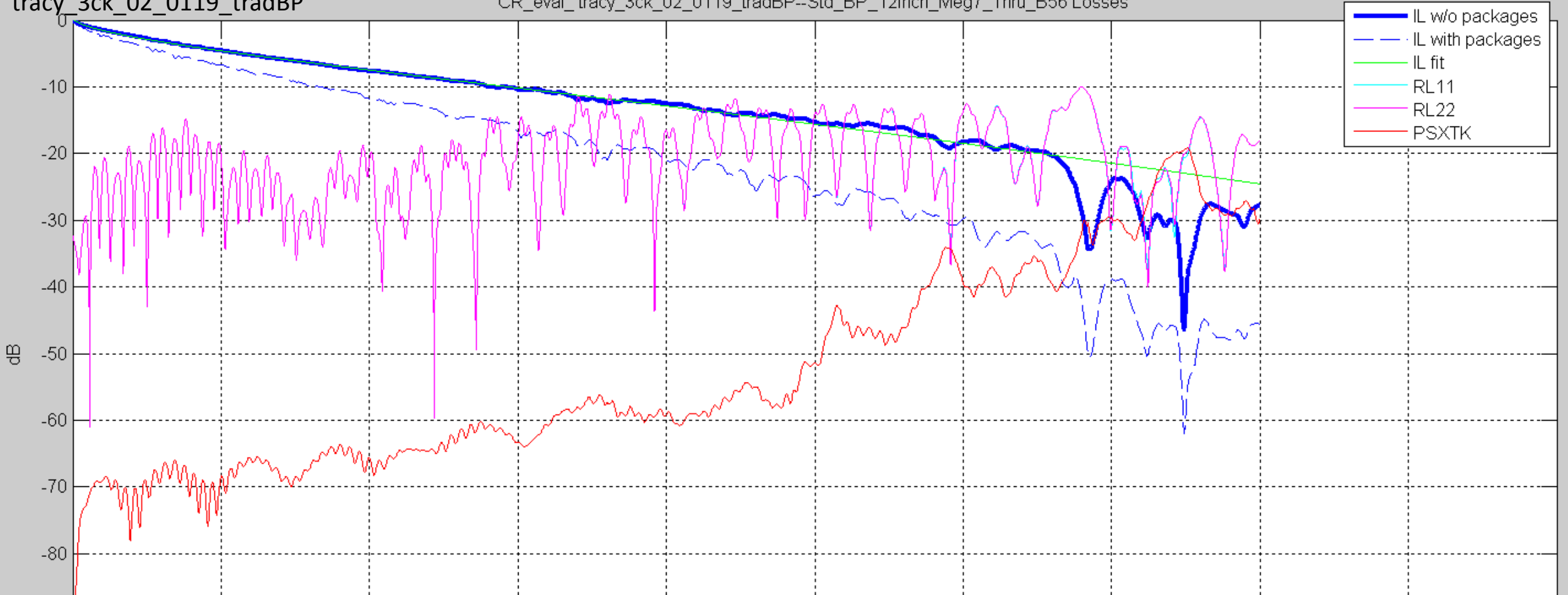
tracy_3ck_02_0119_tradBP
