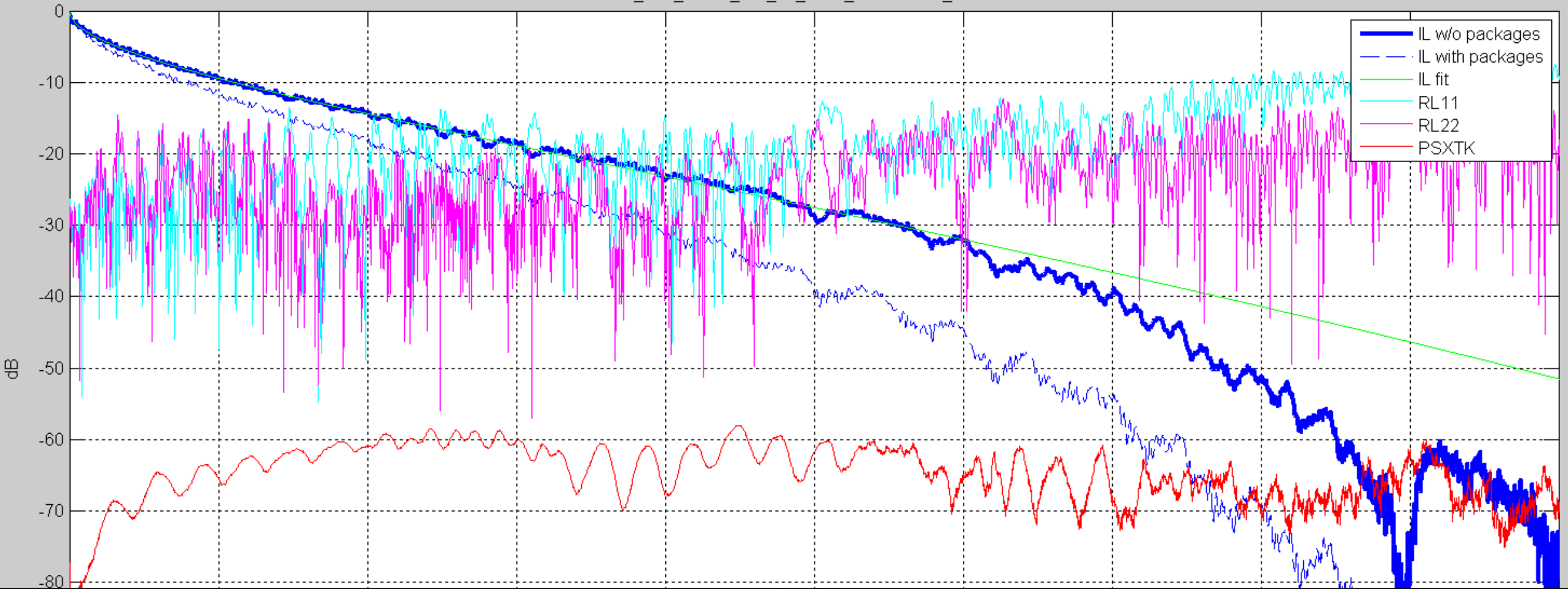
CR_eval_kareti_3ck_01_1118_ortho--Och4_tLosses
