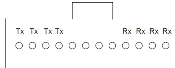
Figure 138-7—Optical lane assignments for 200GBASE-SR4
