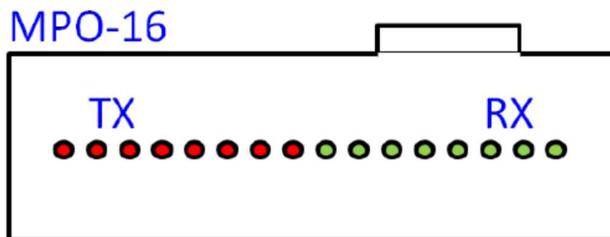
Figure 138-x-400GBASE-SR8 optical lane assignments
