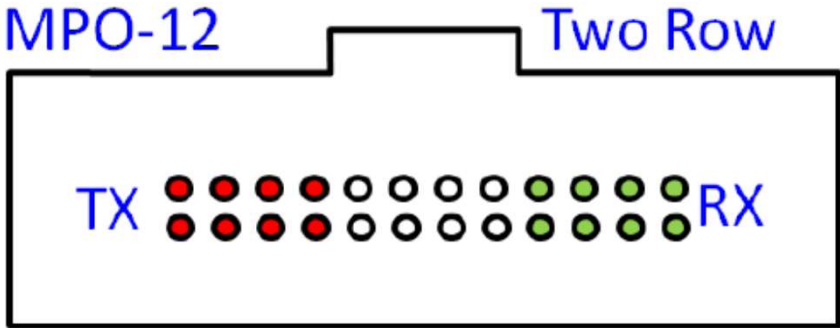
Figure 138-x-400GBASE-SR8 optical lane assignments
