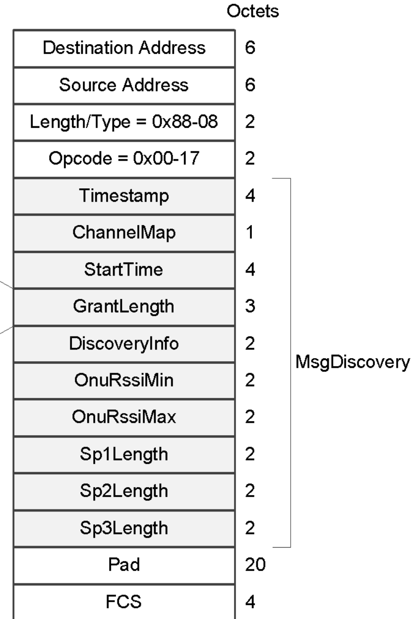
Figure 144-17—DISCOVERY MPCPDU
