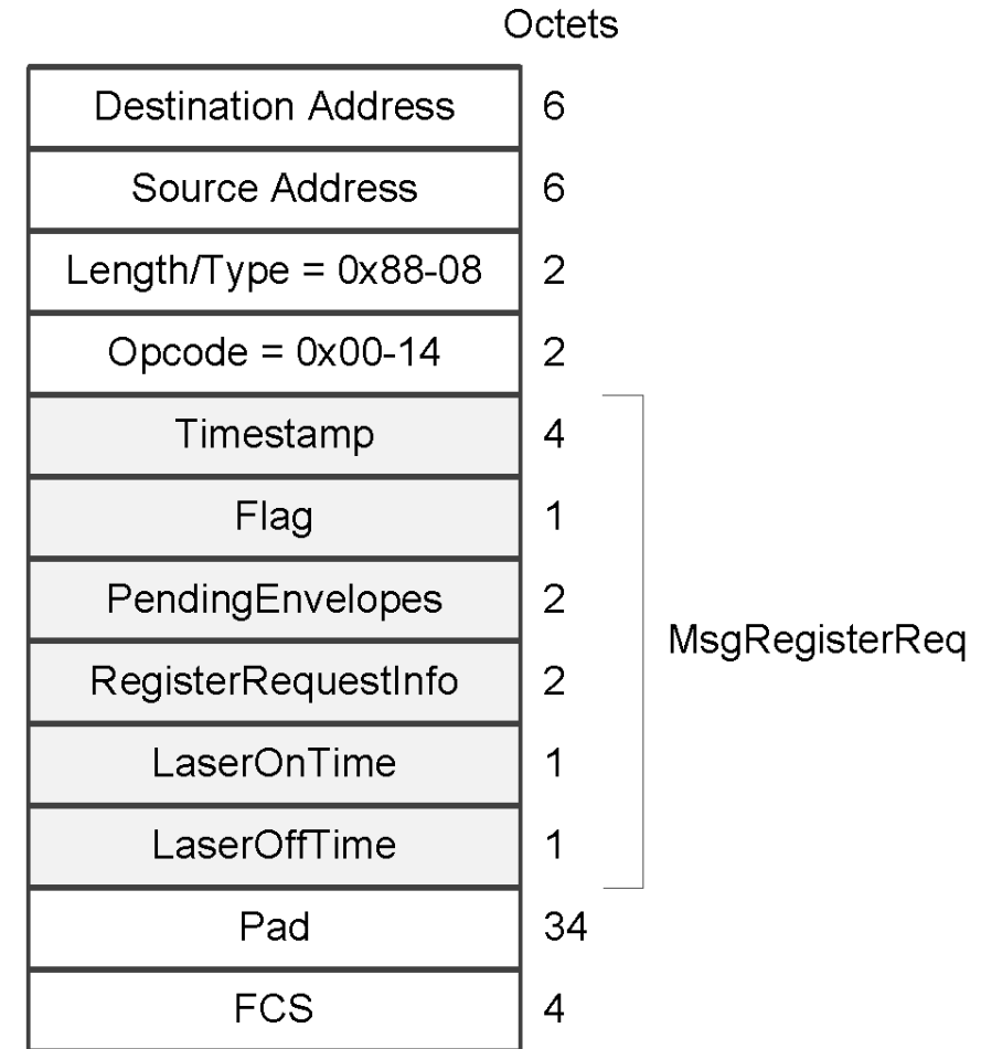
Figure 144-14—REGISTER_REQ MPCPDU
