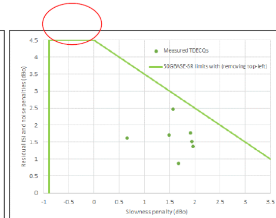
50GBASE-SR, 100GBASE-SR2 and 200GBASE-SR4: limit to 4.5dB
