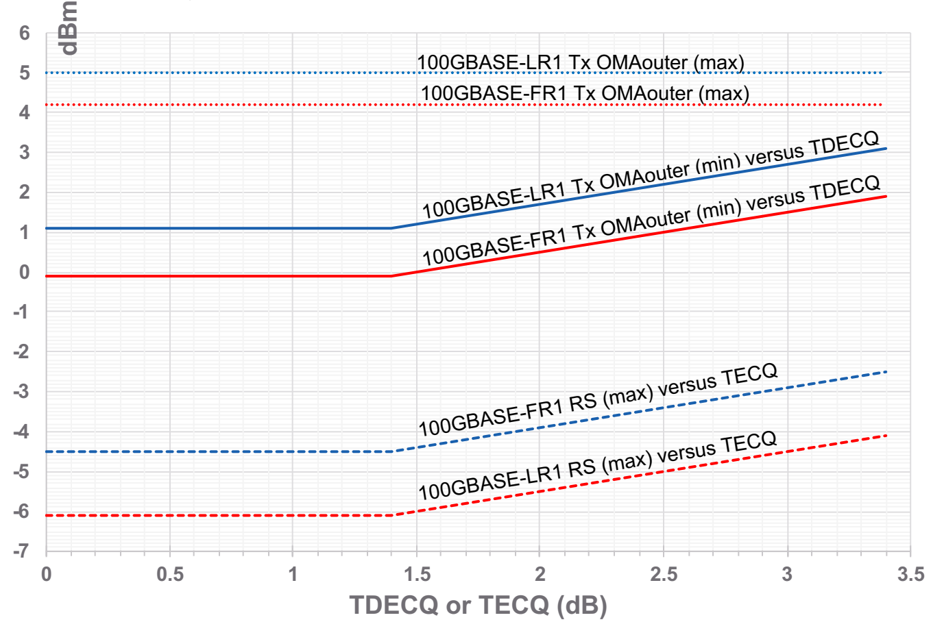
Figure 140-x 100GBASE-FR1 and 100GBASE-LR1 transmitter OMA_{outer} and receiver sensitivity
