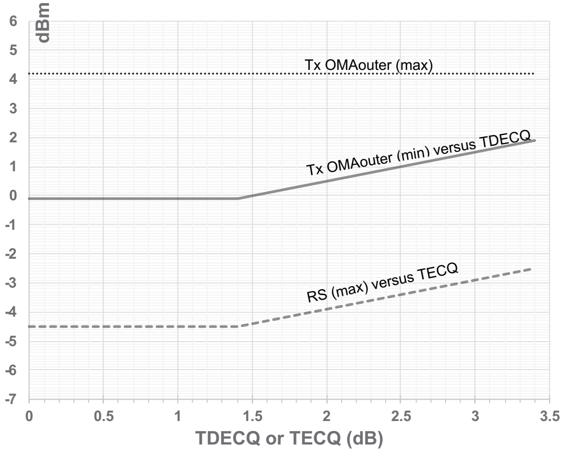
Figure 140-x 100GBASE-FR1 transmitter OMA_{outer} and receiver sensitivity
