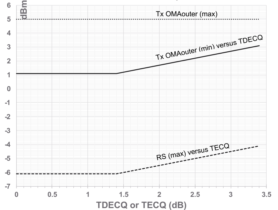
Figure 140-x 100GBASE-LR1 transmitter OMA_{outer} and receiver sensitivity
