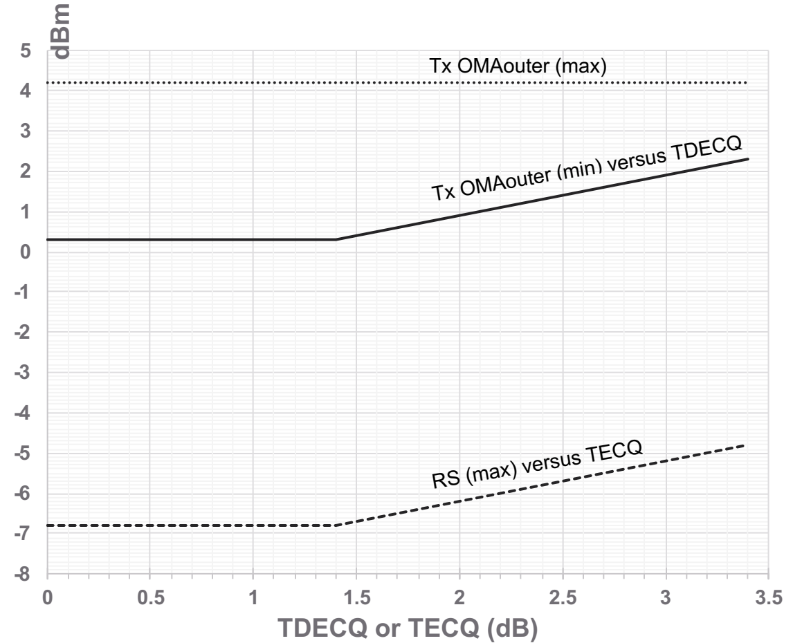
Figure 151-x 400GBASE-LR4-6 transmitter OMA outer and receiver sensitivity
