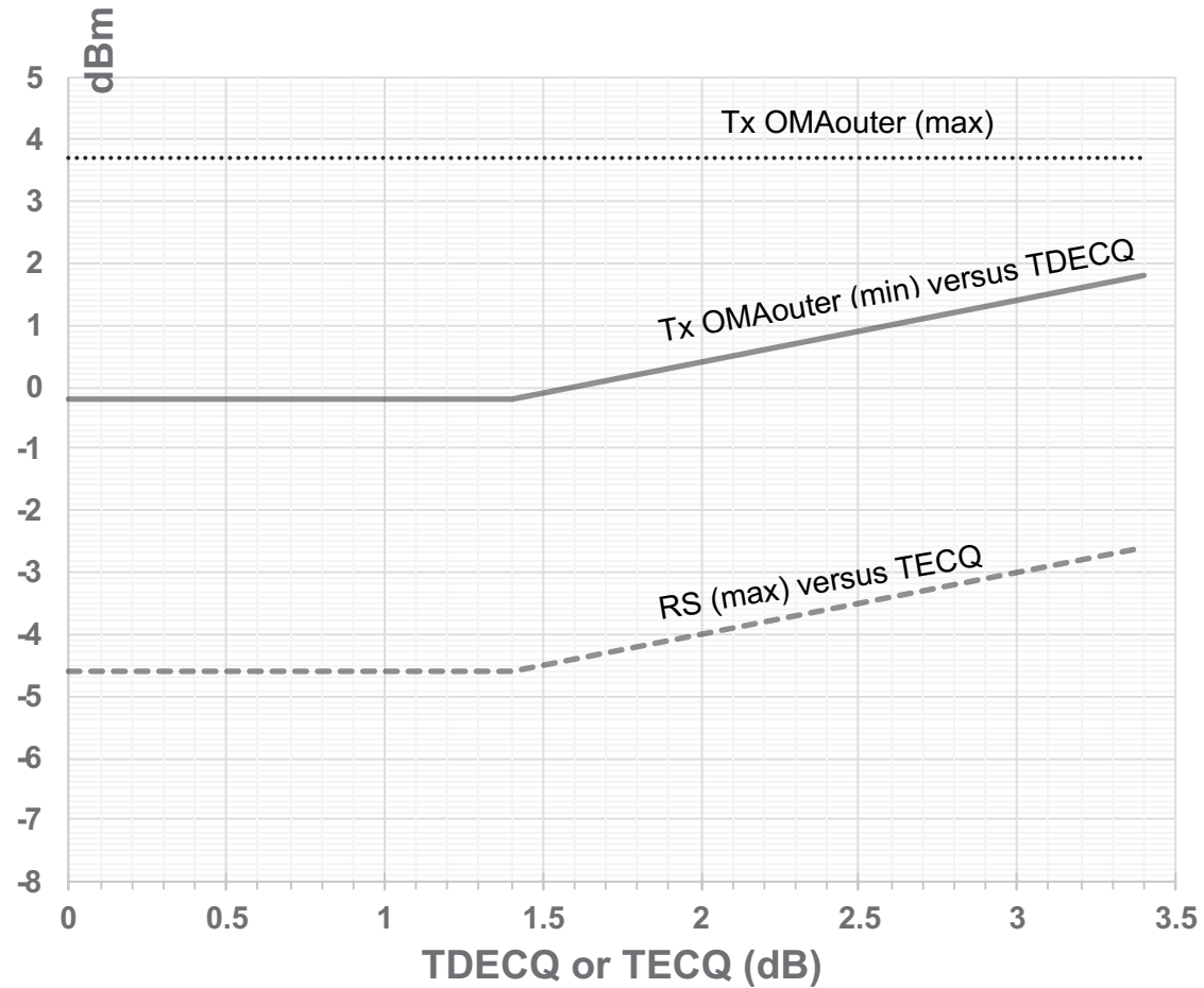
Figure 151-x 400GBASE-FR4 transmitter OMA outer and receiver sensitivity
