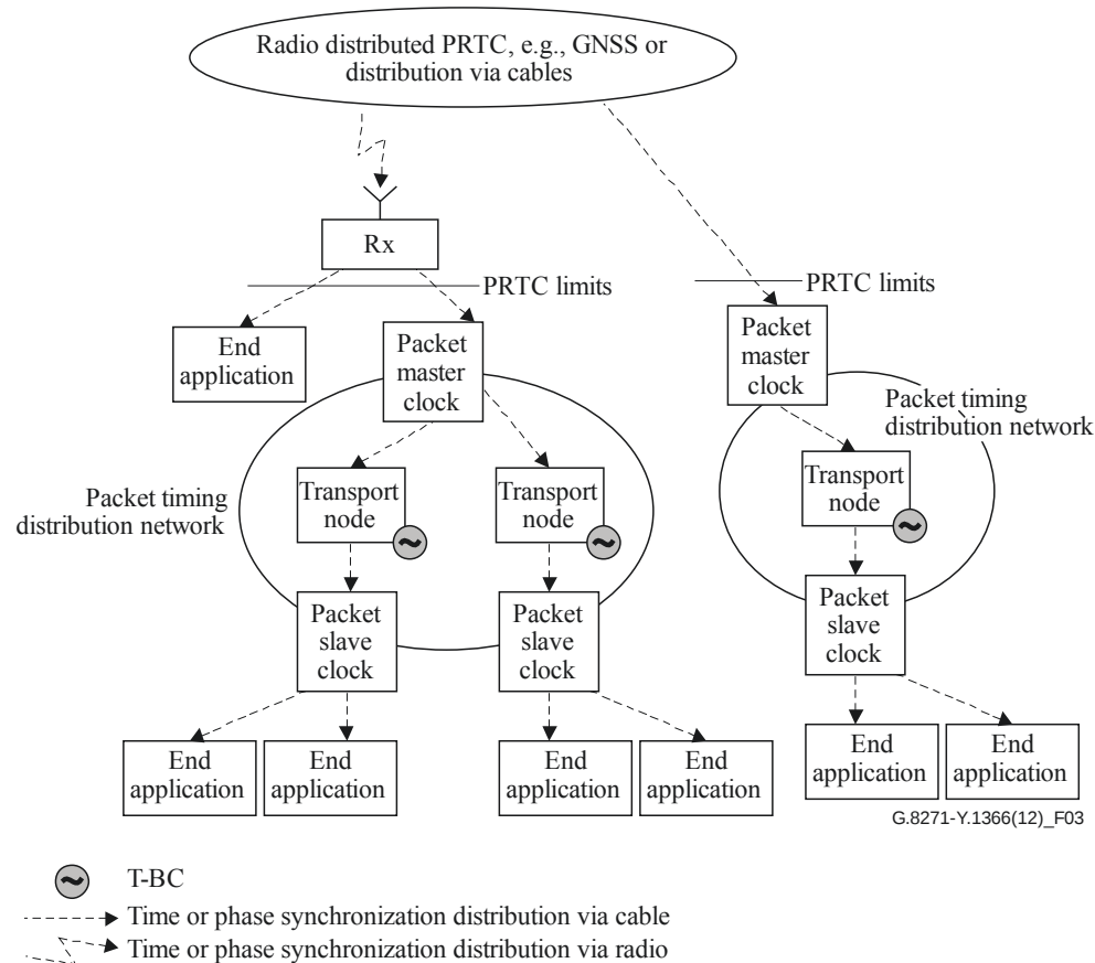
Figure 3/G.8271 - Example of time synchronization distributed via packet based methods
