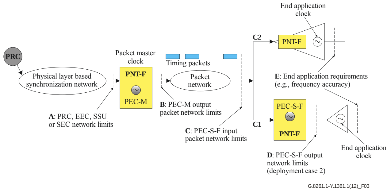
Figure 3/G.8261.1 -Reference Points for network limits
