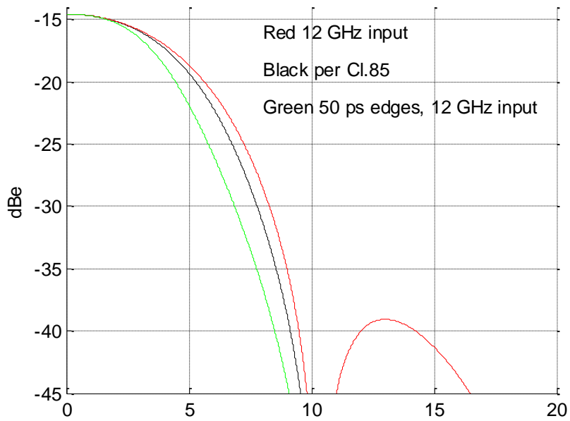
Clause 85 crosstalk weighting functions
