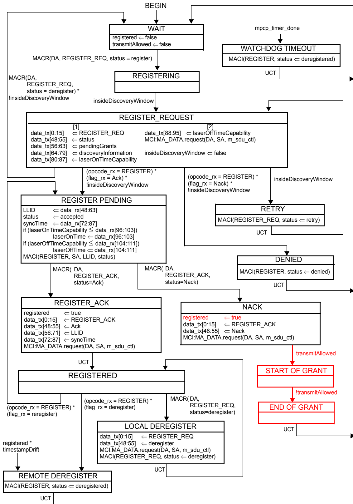
Figure 77-1—Discovery Processing ONU Registration state diagram
