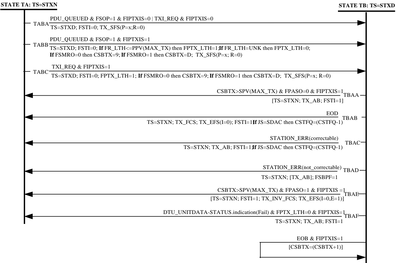
Figure L-2 Transmit FSM
