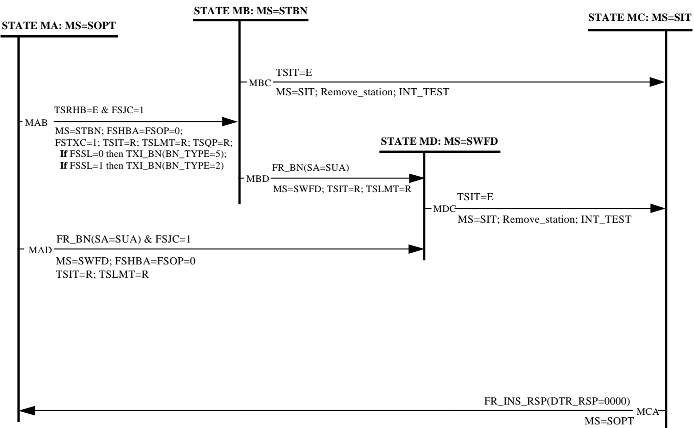
Figure L-3 - MONITOR FSM
