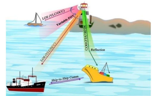
Seaside Environment Lighthouse-to-Ship/Ship-to-Ship
