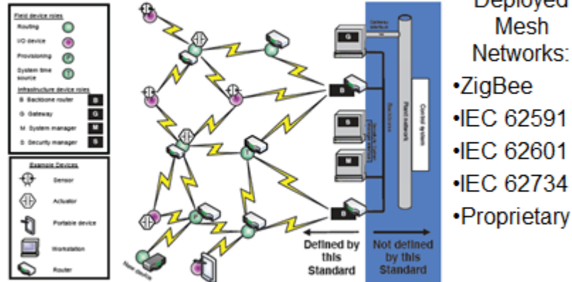
Figure 1 – Standard-compliant network Example of Deployed Mesh Networks
