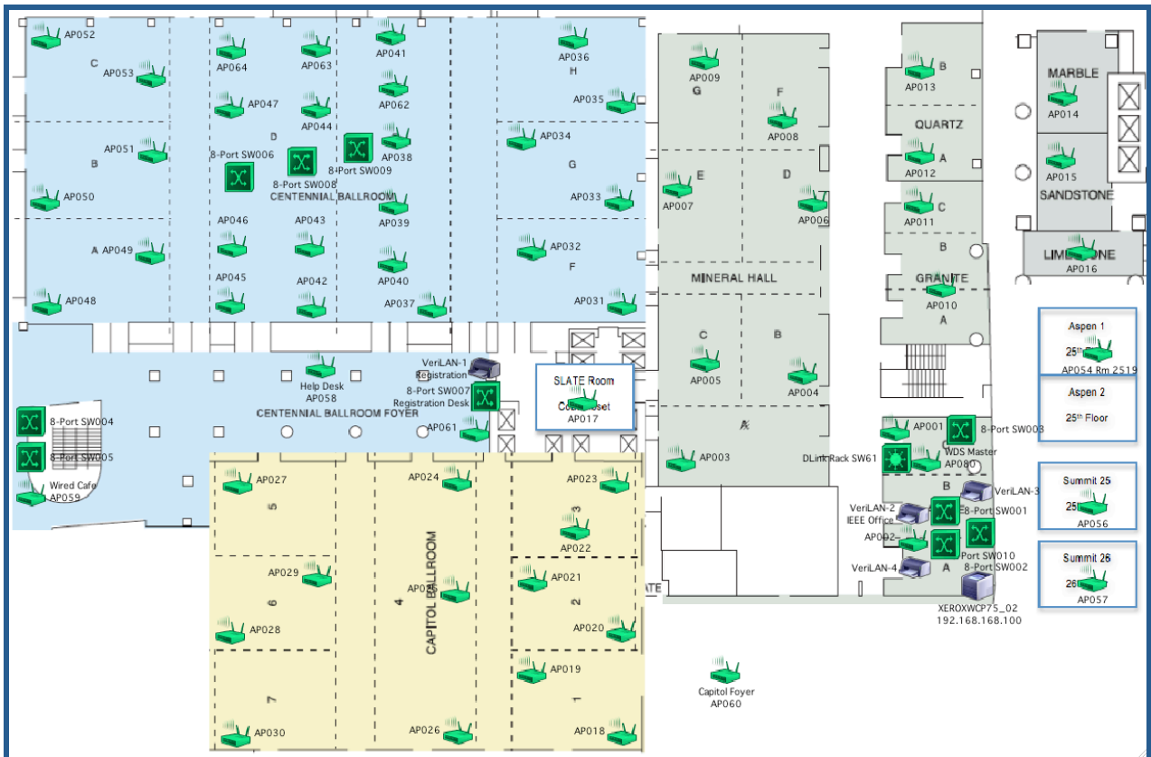
Figure 5. Wireless Access Point Deployment Plan
