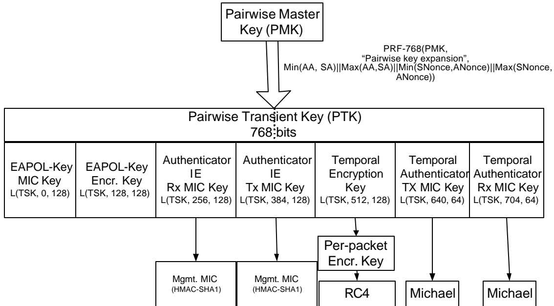
Figure 5—Complete TKIP Pairwise Key Hierarchy for use with Authenticator IE
