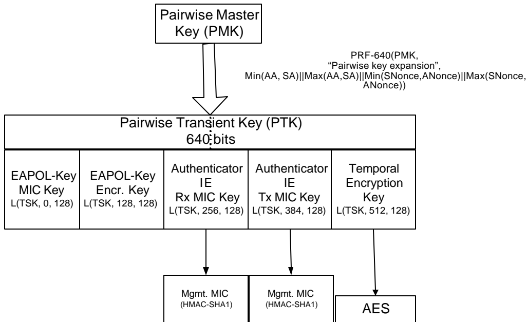
Figure 6—Complete WRAP Pairwise Key Hierarchy for use with Authenticator IE
