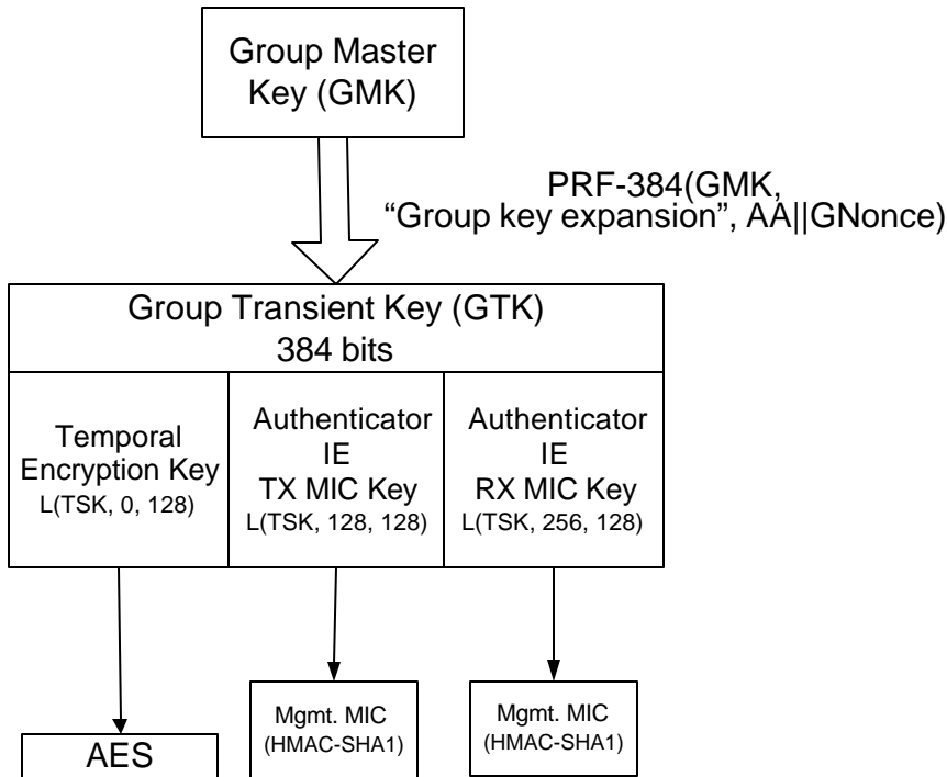
Figure 8—Complete WRAP Group Key Hierarchy for use with Authenticator IE
