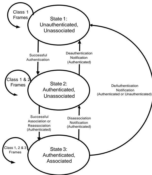
Figure 3 – Relationship between state variables and services
