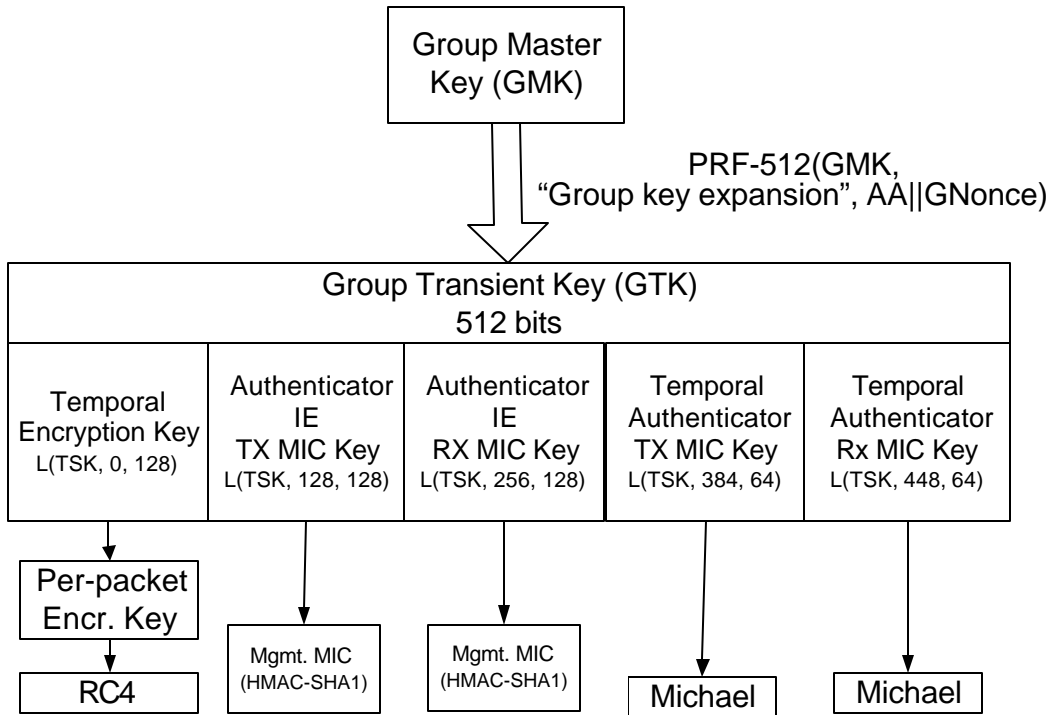
Figure 7—Complete TKIP Group Key Hierarchy for use with Authenticator IE
