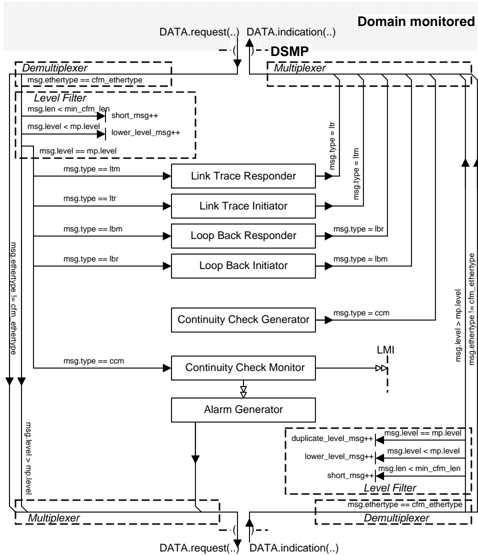
Figure 13—Maintenance End Point monitoring at a DSMP
