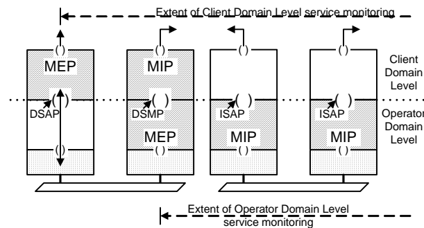
Figure 6—Adding Maintenance Point Entities
