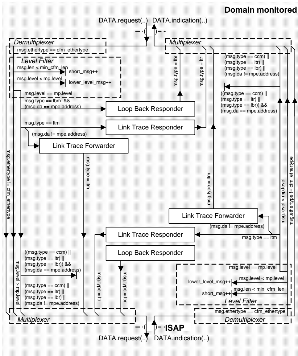
Figure 14—MIP supporting domain monitoring at an ISAP
