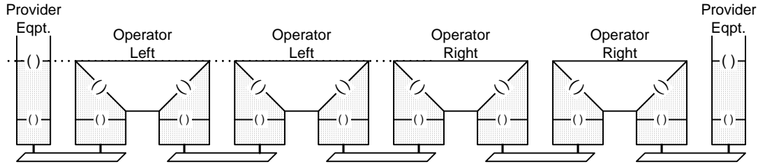
Figure 7—Concatenated networks
