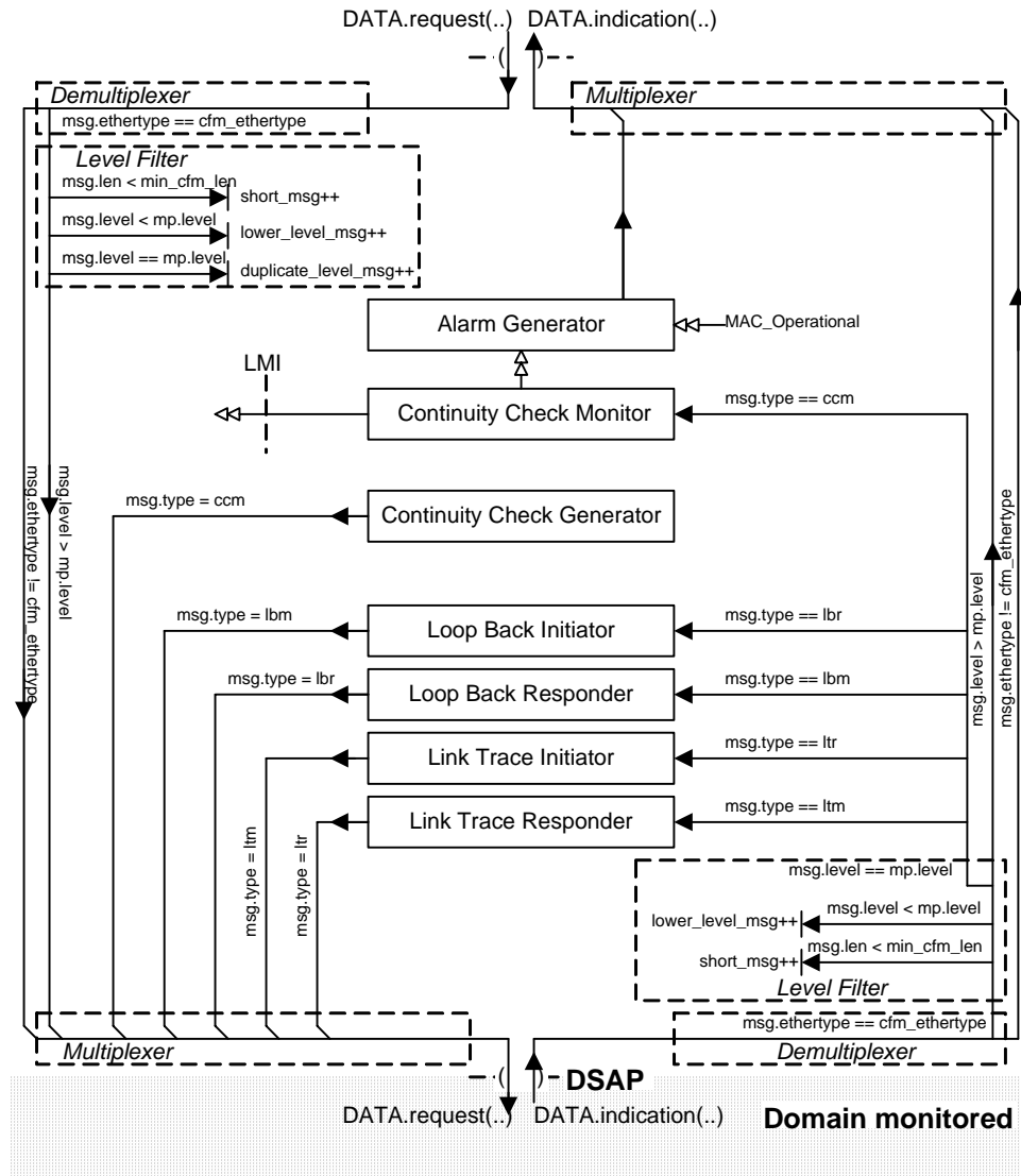
Figure 12—Maintenance End Point monitoring at a DSAP
