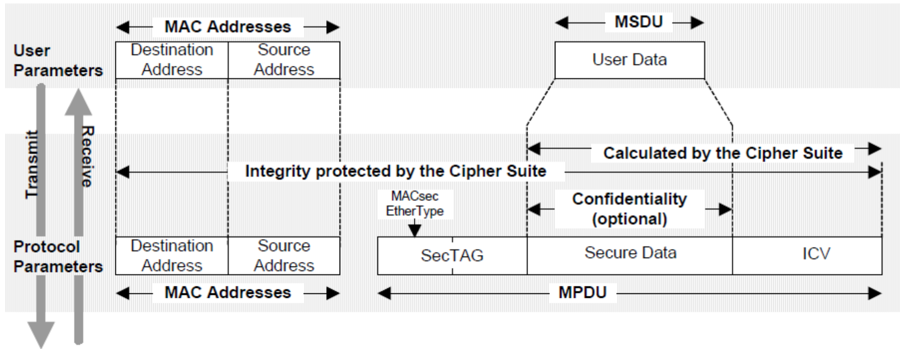
Figure 8-1—MACsec
