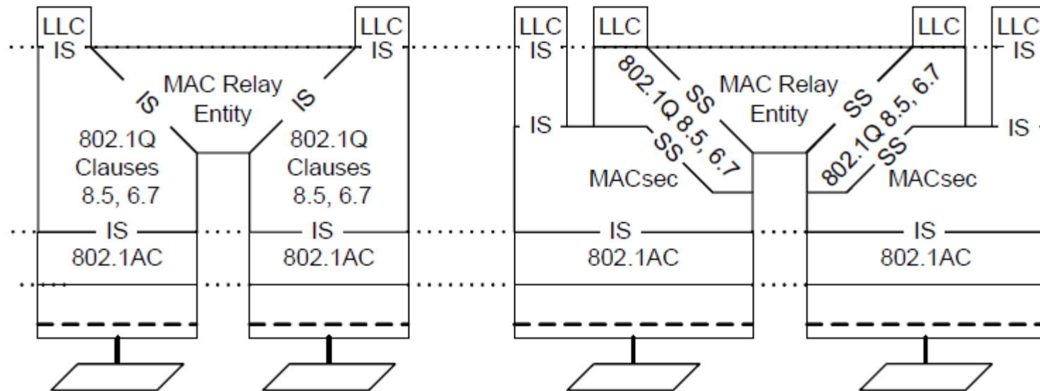
Figure 11-6—Addition of MAC Security to a VLAN-aware MAC Bridge
