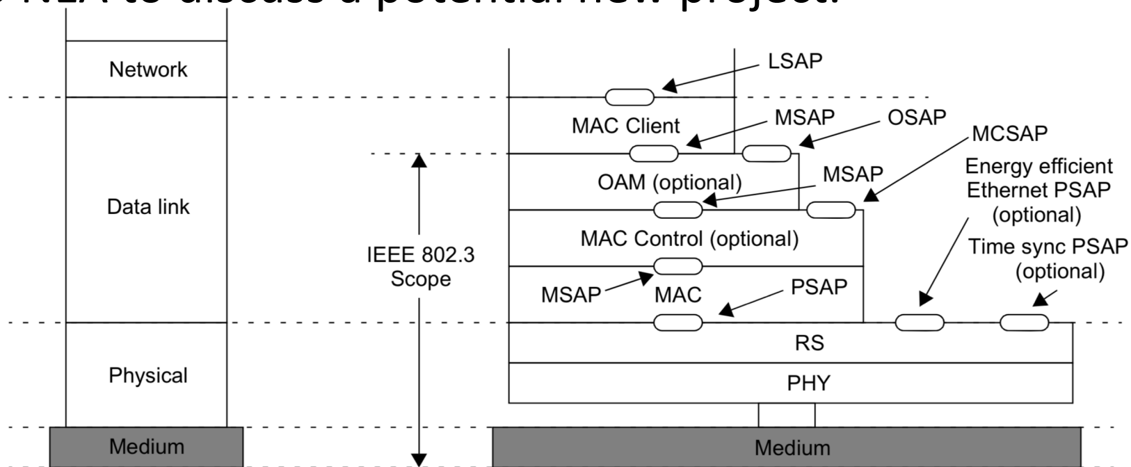
Figure B.2—The RM for IEEE 802.3 point-to-point stations
