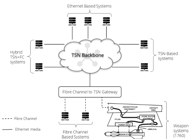
670 671 Figure 5 Fibre Channel over TSN Backbone
