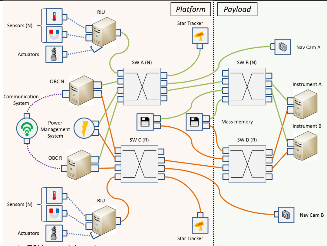
Figure 4 - TSN potential topology
