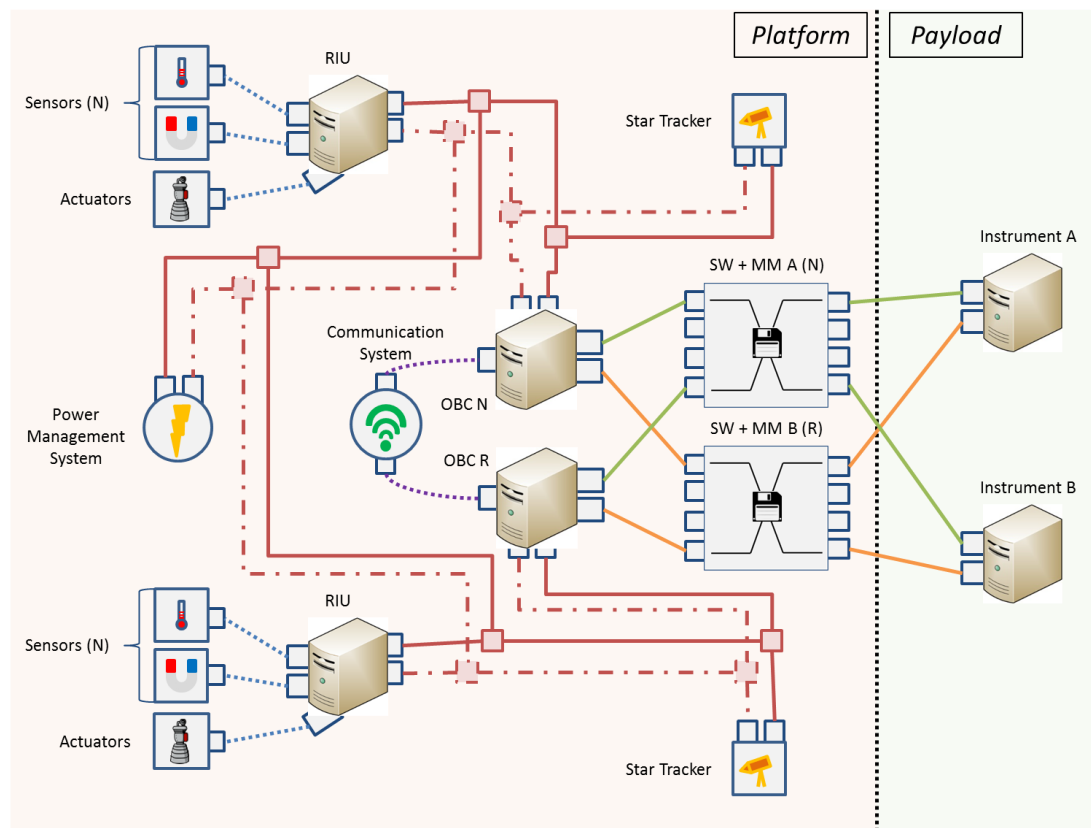
571 Figure 3 - Current Network Topology 572
