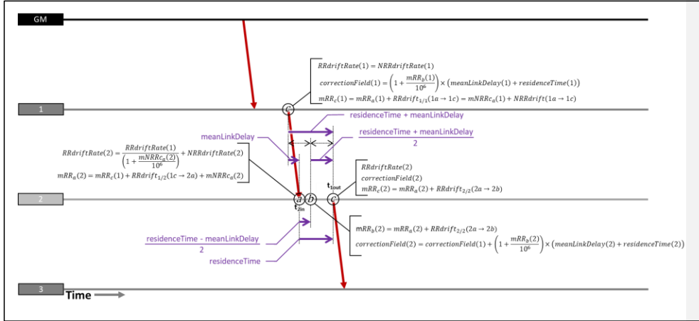
Figure 104: RR Drift Tracking and Error Compensation Calculations
