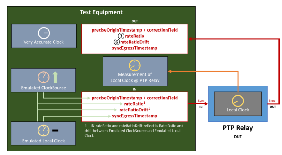
Figure 102: Approach to Testing Normative Requirements for PTP Relay Instance - 2
