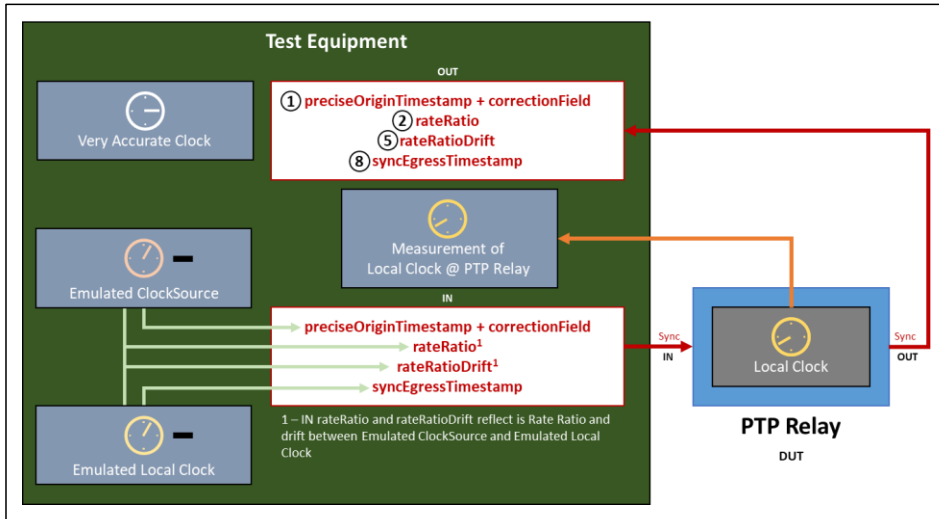
Figure 101: Approach to Testing Normative Requirements for PTP Relay Instance - 1
