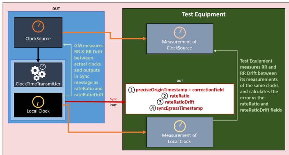
Figure 100: Approach to Testing Normative Requirements for Grandmaster PTP Instance
