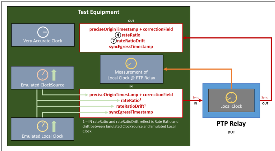
Figure 103: Approach to Testing Normative Requirements for PTP Relay Instance - 3
