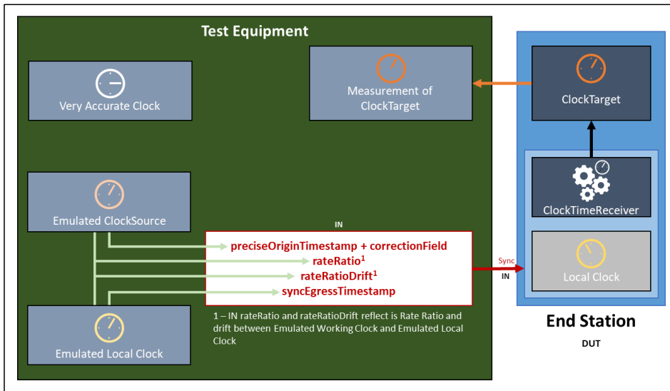
Figure 104: Approach to Testing Normative Requirements for PTP End Instance
