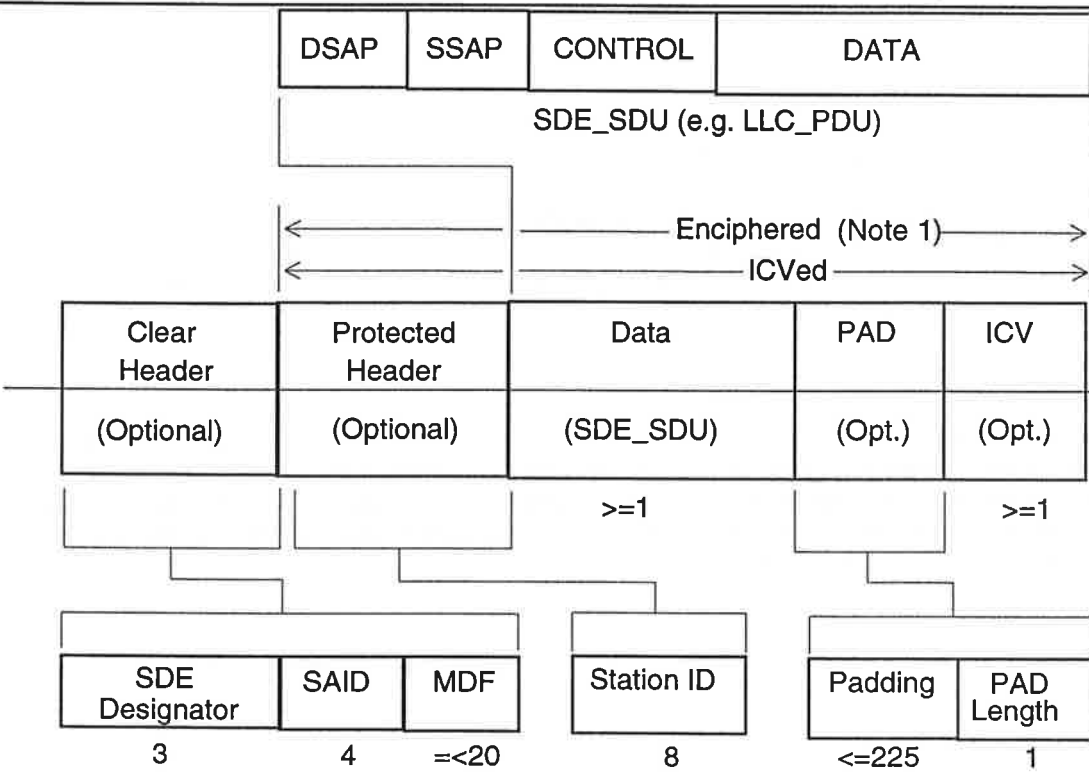
Figure 3-1: Construction of the Structure of SDE_PDU
