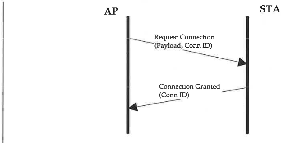
Figure 3-5: Connection Initiated by AP
