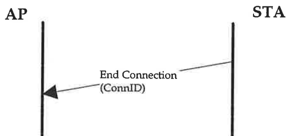
Figure 3-7: End Connection
