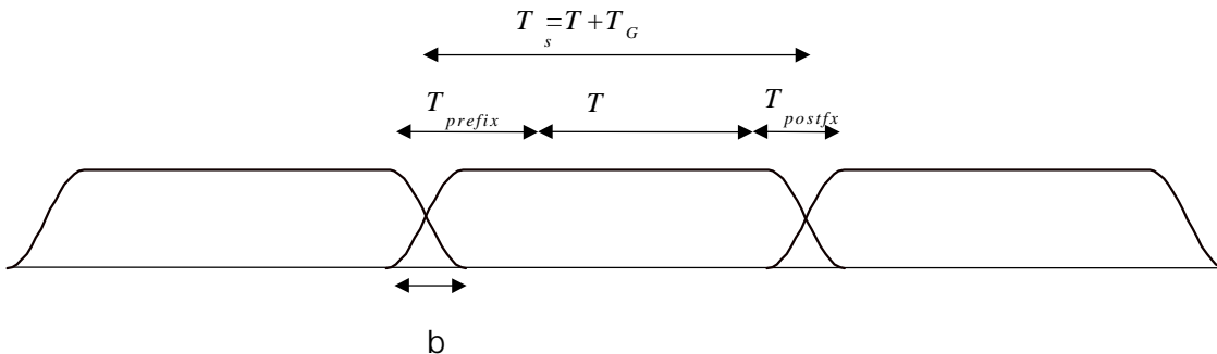
Figure 116: OFDM cyclic extension and windowing.
