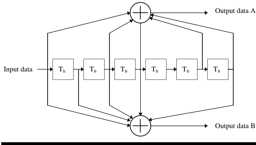
Figure 111, Convolutional Encoder
