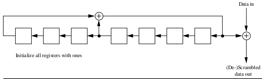
Figure 110, Data Scrambler
