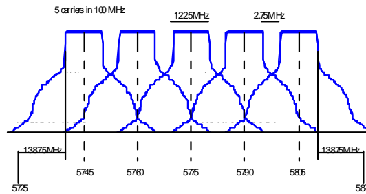
Figure 114, OFDM PHY Frequency Channel Plan
