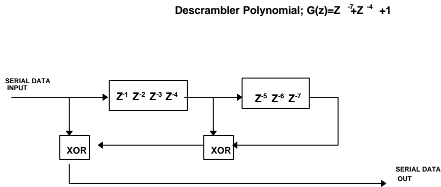
Figure 92, Data Descrambler
