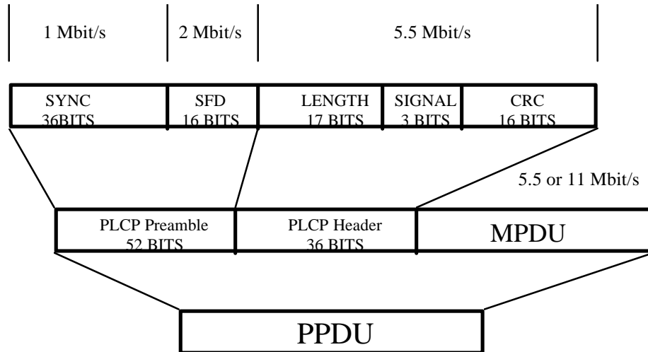
Figure 89, Short, High Rate only, PLCP Frame Format
