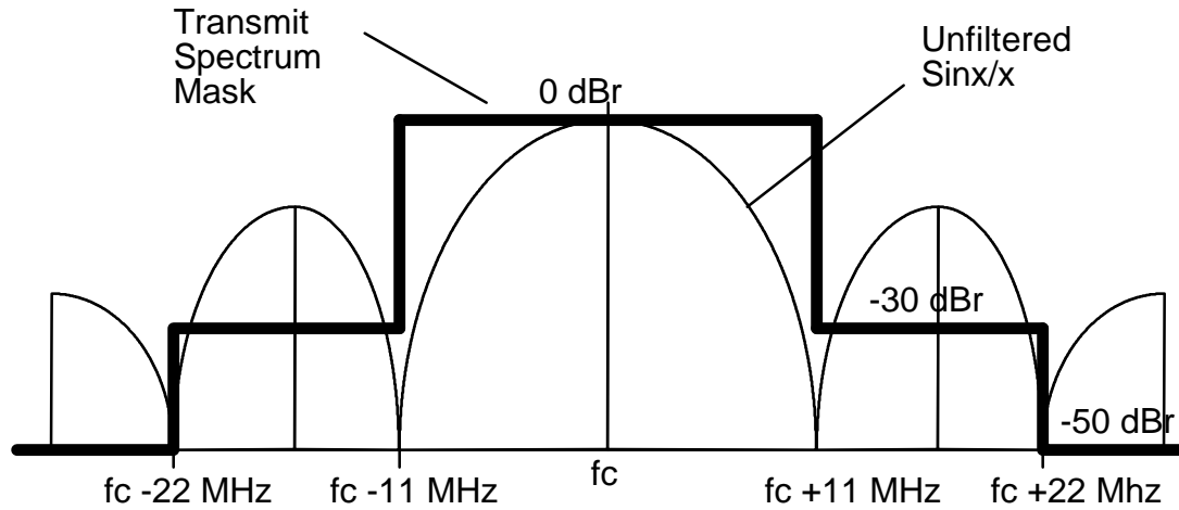
Figure 98, Transmit Spectrum Mask
