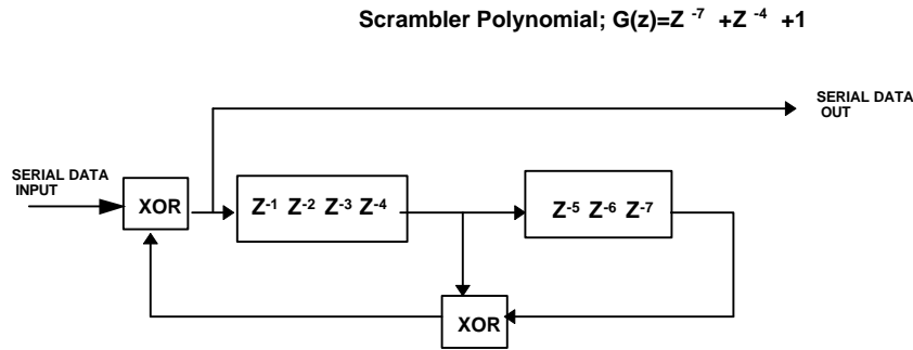
Figure 91, Data Scrambler
