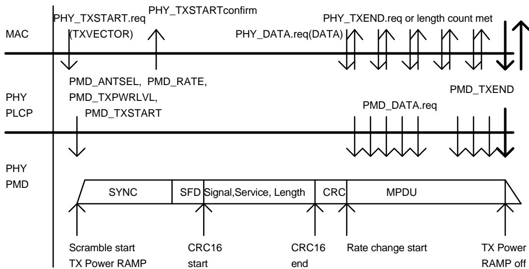
Figure 93, PLCP Transmit Procedure
