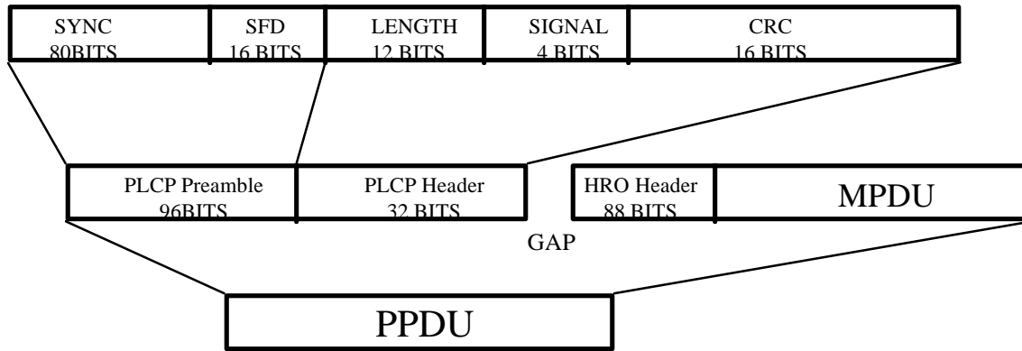
Figure 90, FH interoperable PLCP Frame Format
