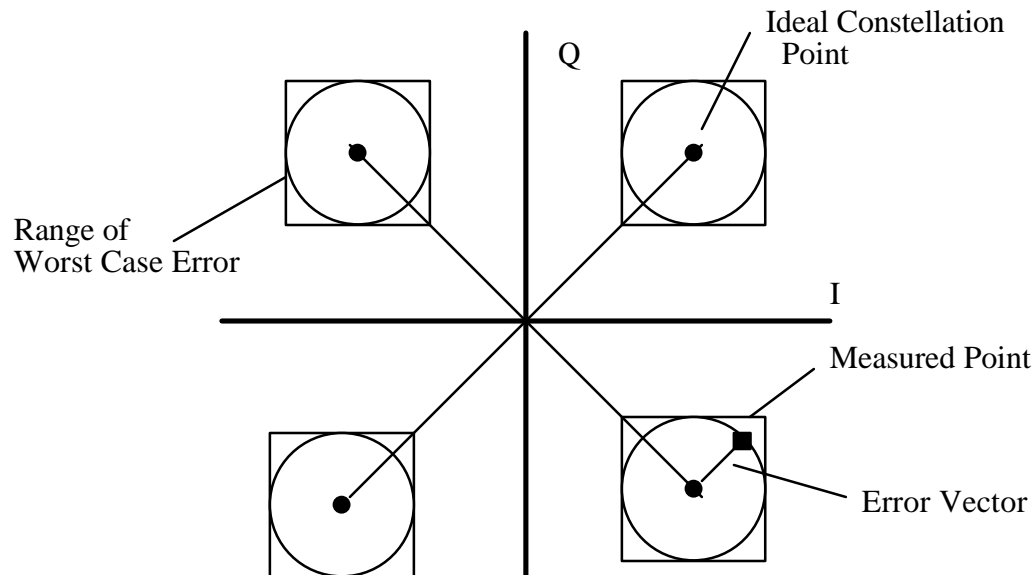
Figure 101, Modulation Accuracy Measurement Example
