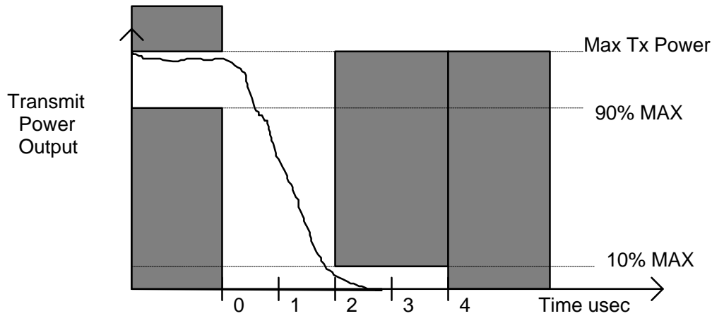
Figure 100, Transmit Power Down Ramp
