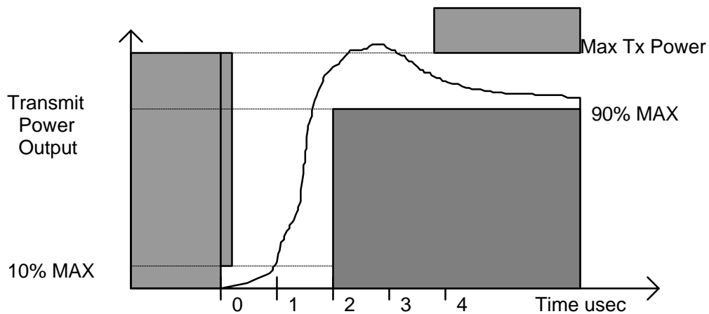
Figure 99, Transmit Power On Ramp
