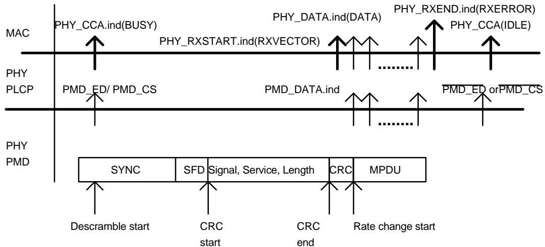
Figure 95, PLCP Receive Procedure
