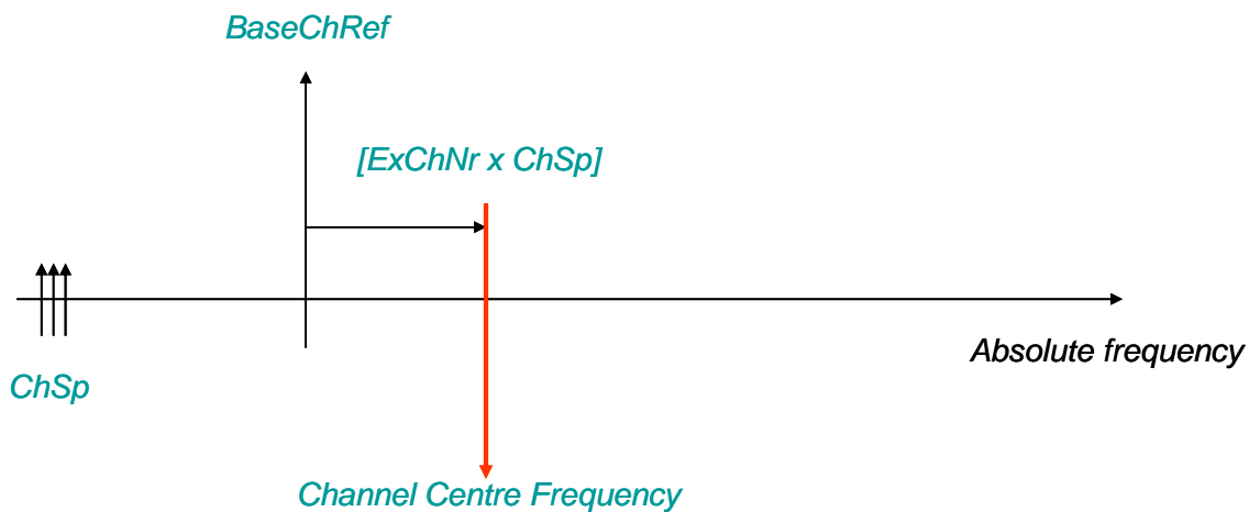
Figure xyz Representation of 'Channel Centre Frequency' calculation.
