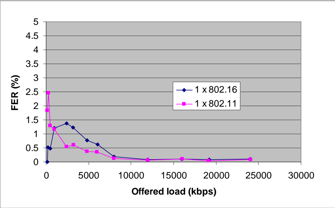
Figure 6 Scenario E – Occupancy and FER against offered load.
