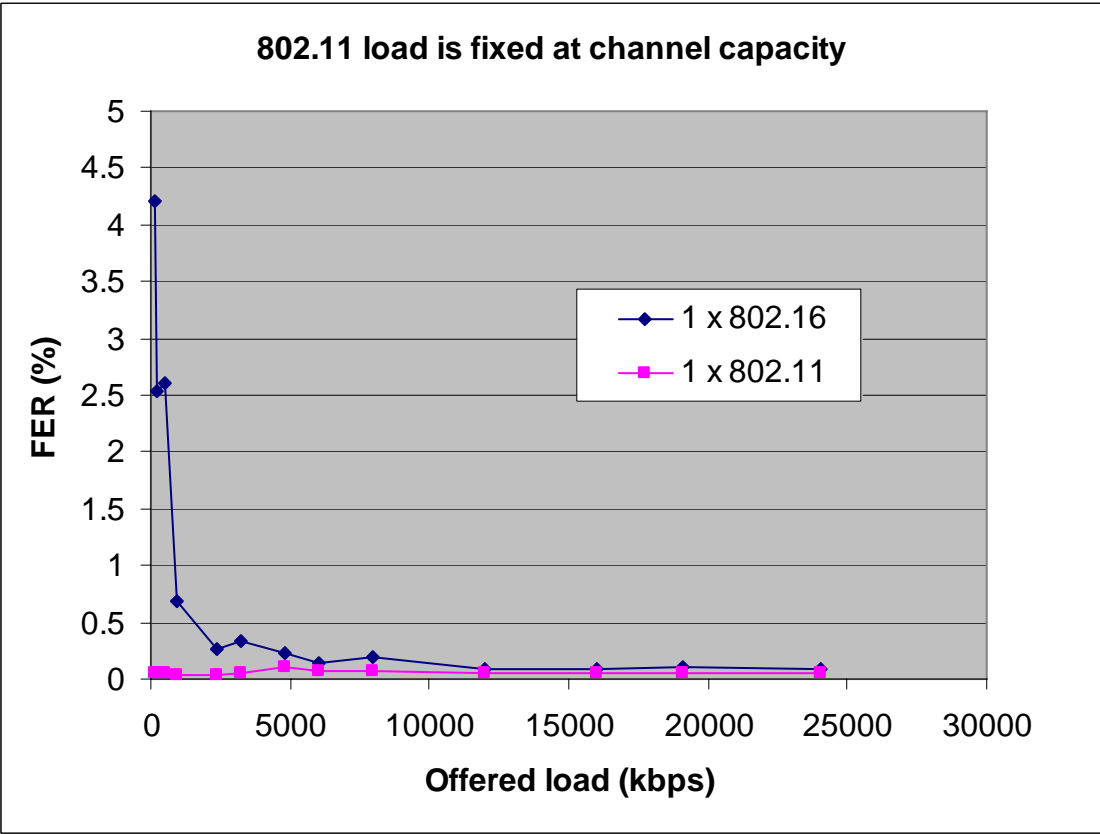
Figure 15 Scenario O – Occupancy and FER against offered load. 802.11 load fixed at channel
