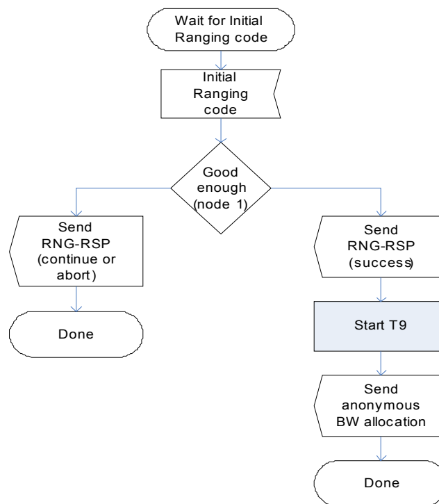
Figure 87 CDMA Initial Ranging -- BS
