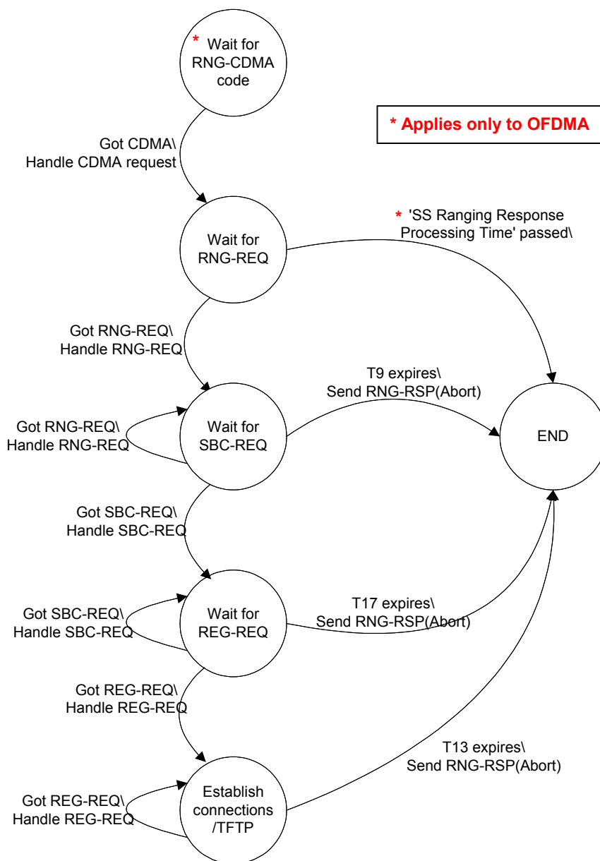
Figure 70a – Network entry state-machine BS side.
