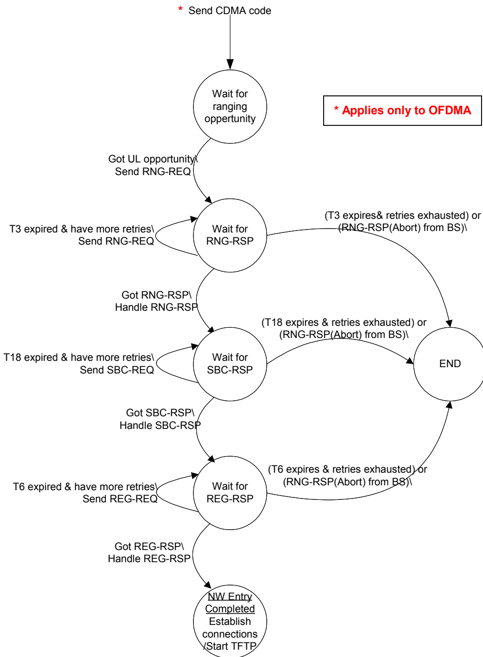
Figure 70b – Network entry state-machine MS/SS side.
