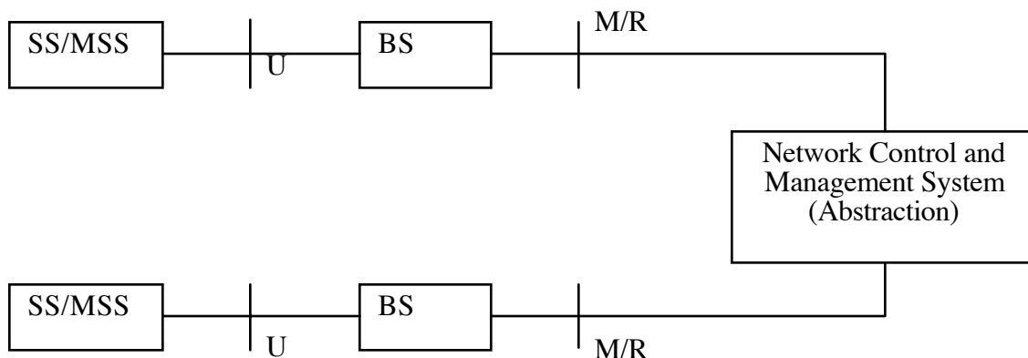
Figure 1: Logical Network Reference Model (Informational)
