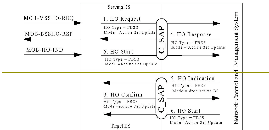
Figure 329—Example Primitive Flow of Active Set Update (Add)
