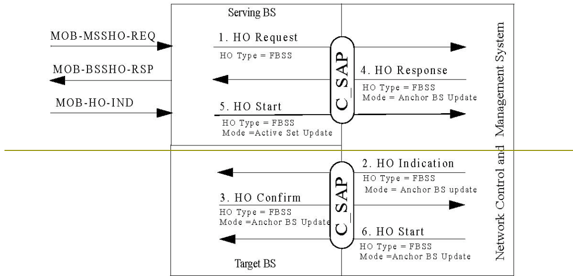
Figure 331—Example Primitive Flow of Anchor BS Update (Using MAC messages)
