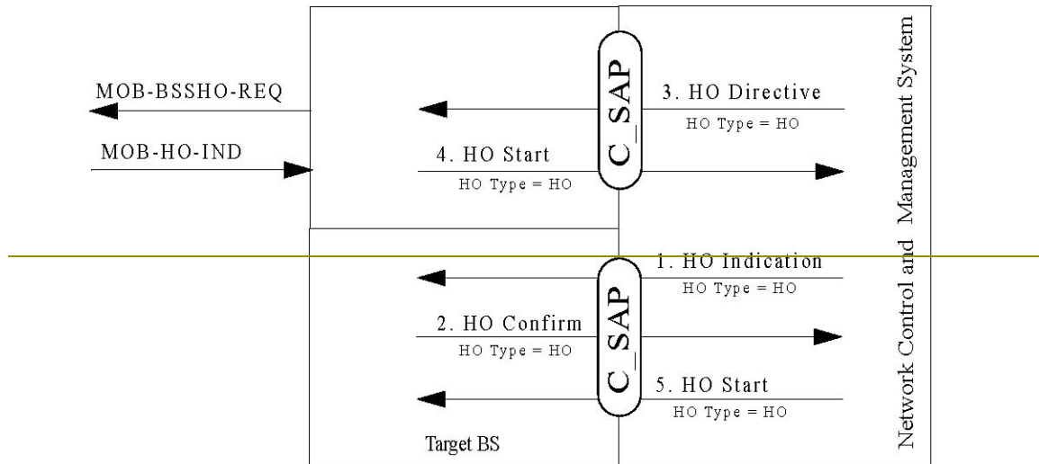
Figure 327—Example Primitive Flow of HO Initiated by BS
