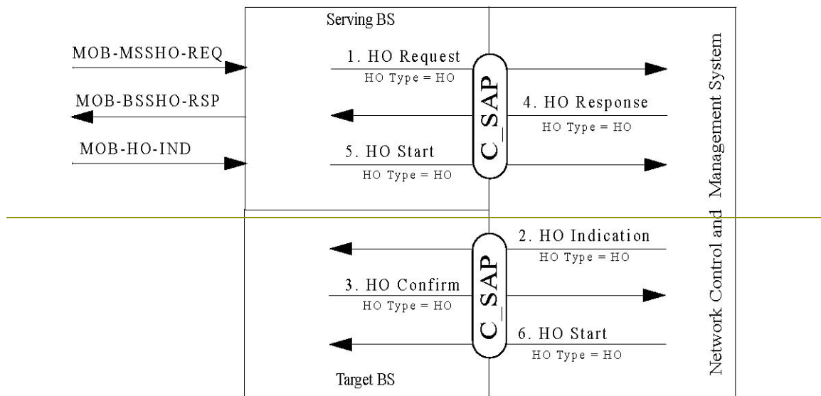
Figure 326—Example Primitive Flow of HO Initiated by MS
