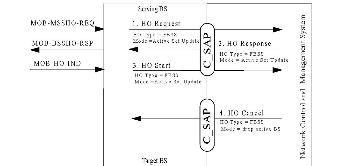
Figure 330—Example Primitive Flow of Active Set Update (Drop)
