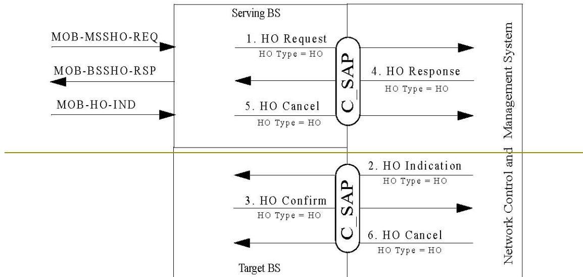
Figure 328—Example Primitive Flow of HO Cancel
