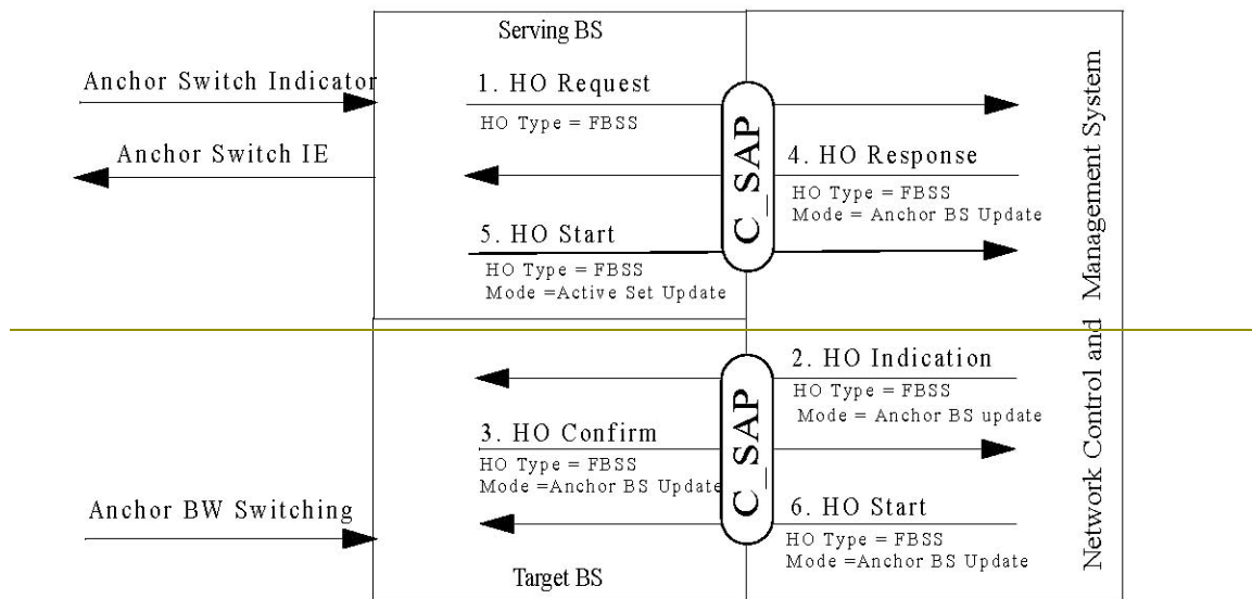
Figure 332—Example Primitive Flow of Anchor BS Update (Using selection feedback mechanism)
