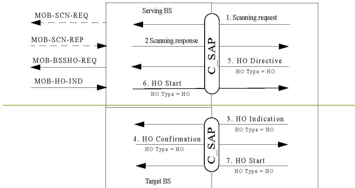
Figure 325—Example Primitive Flow of HO initiated by BS
