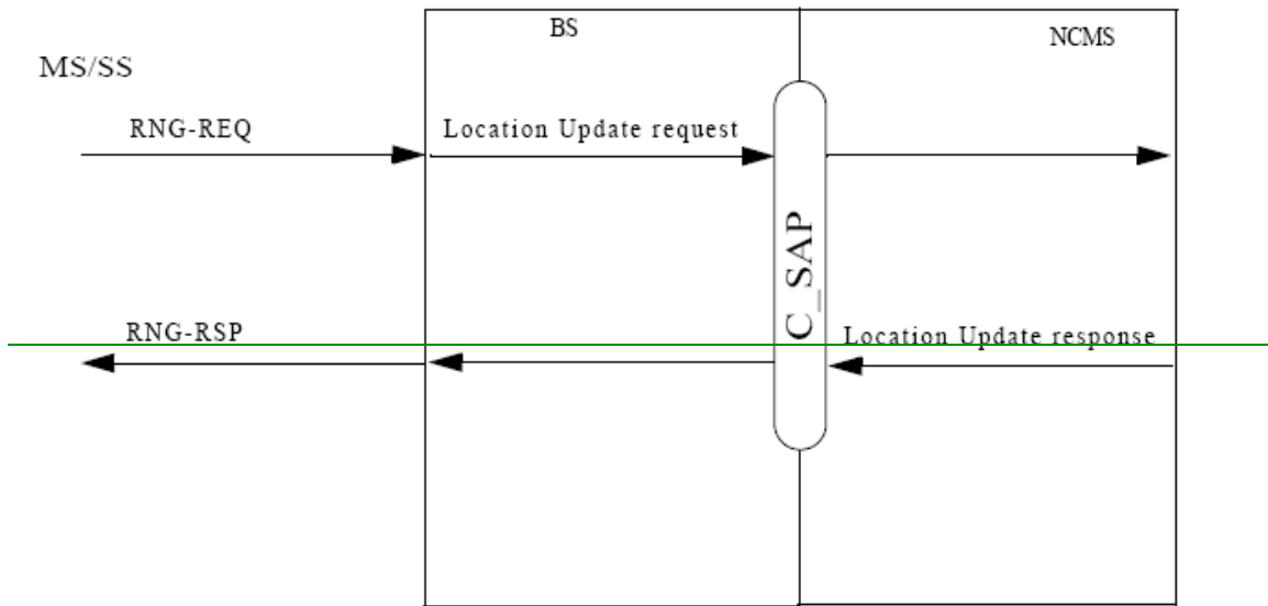
Figure 324— Location Update Primitives
