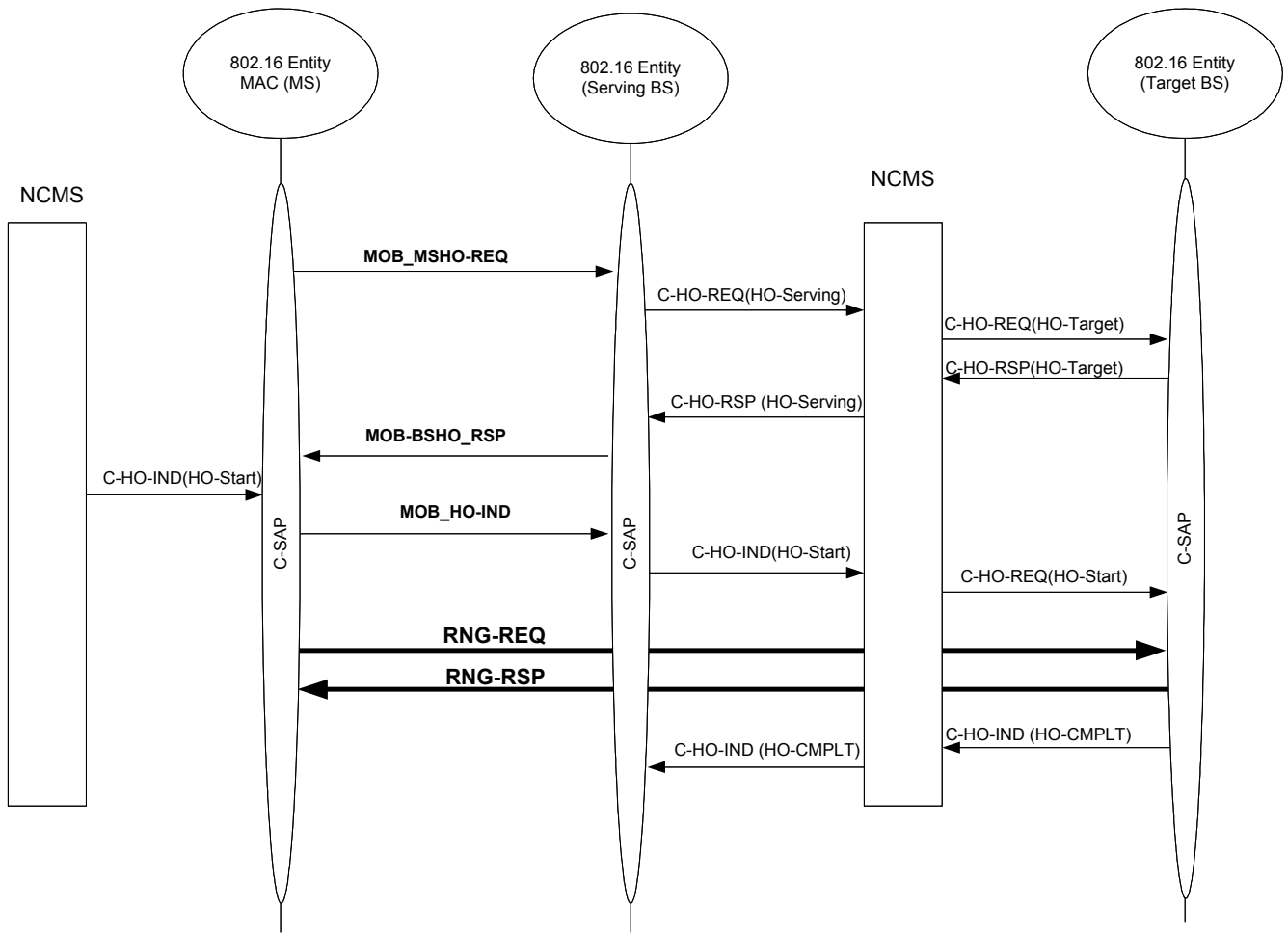
Figure F8 – End-to-End HO exchange between MS, Serving BS and Target BS
