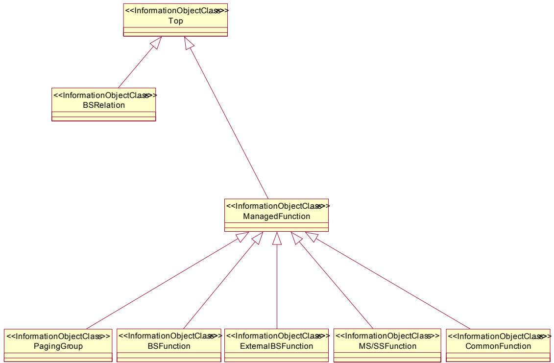
Figure 12 General Inheritance Diagram
