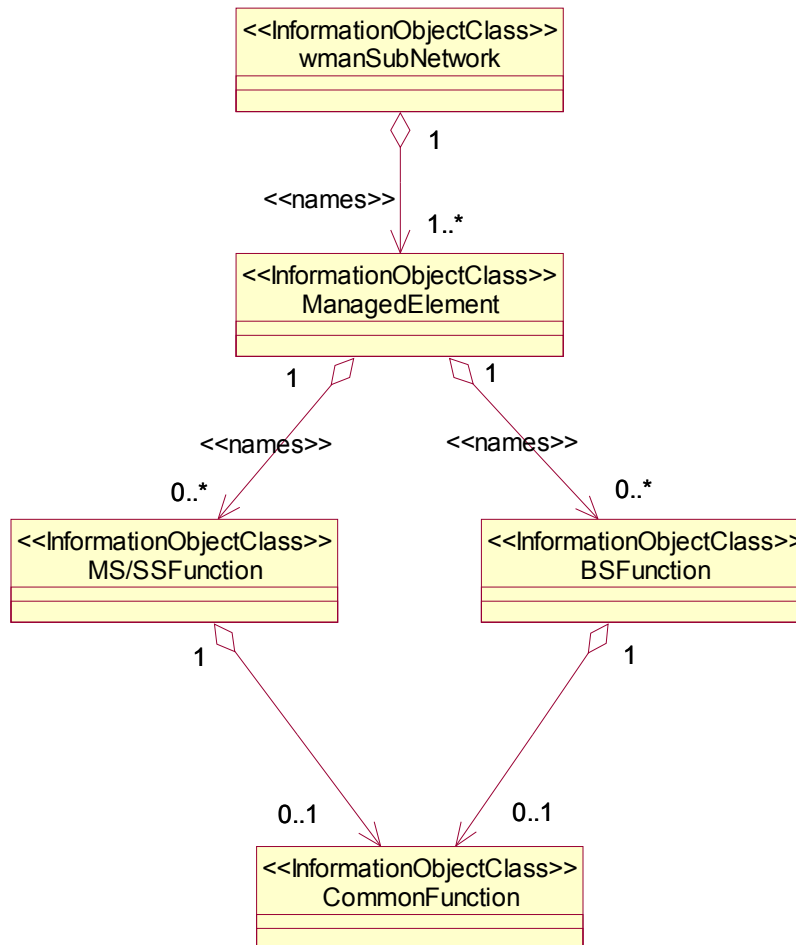
Figure 6 General Containment/Naming Diagram
