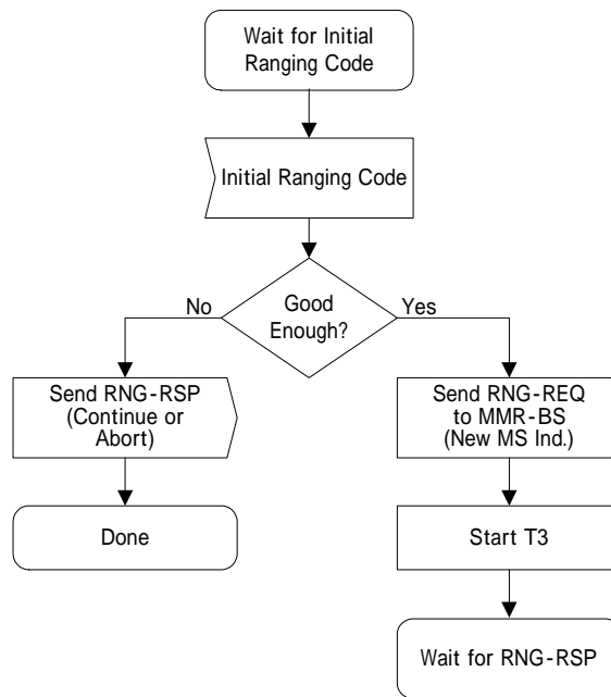
Figure-xxx MS CDMA ranging - RS
