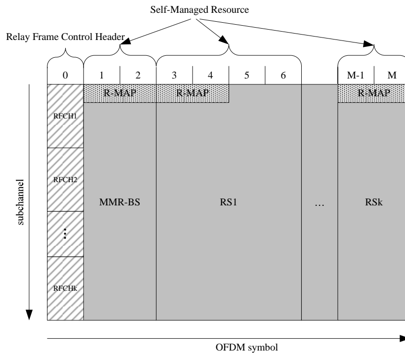
Figure 6 Accommodation of multiple RSs in the BRZ
