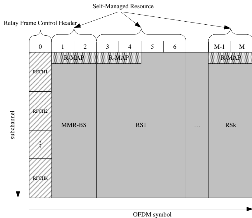
Figure 14 Accommodation of multiple RSs in the BRZ
