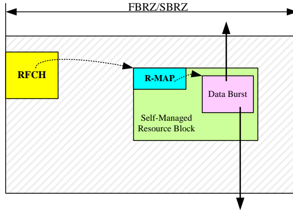
Figure 5 Example of zoomed BRZ
