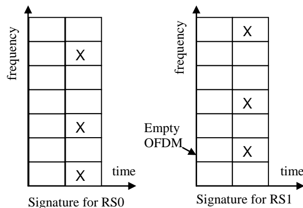
Figure 1. Example of signatures for two RSs. On the carriers marked with “X” energy is transmitted.
